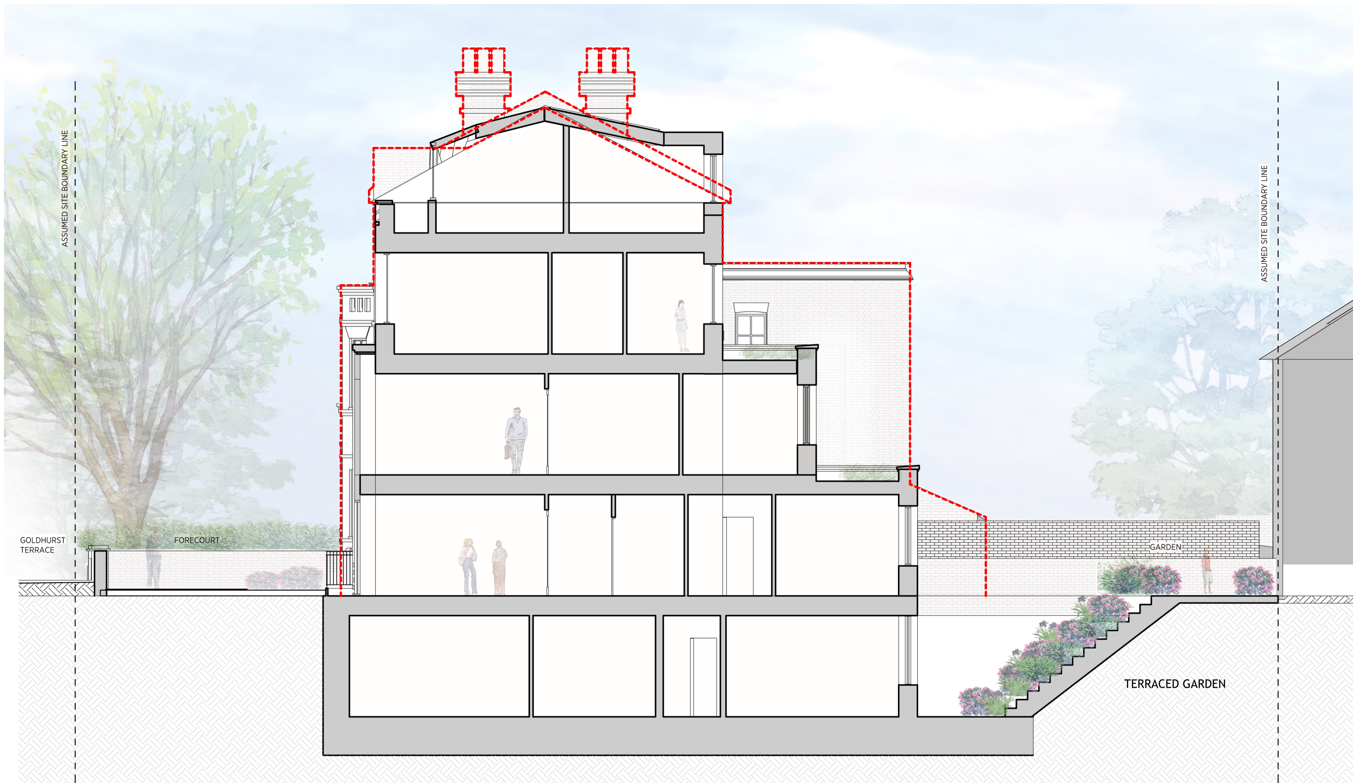
1 SECTION CC 1:50
