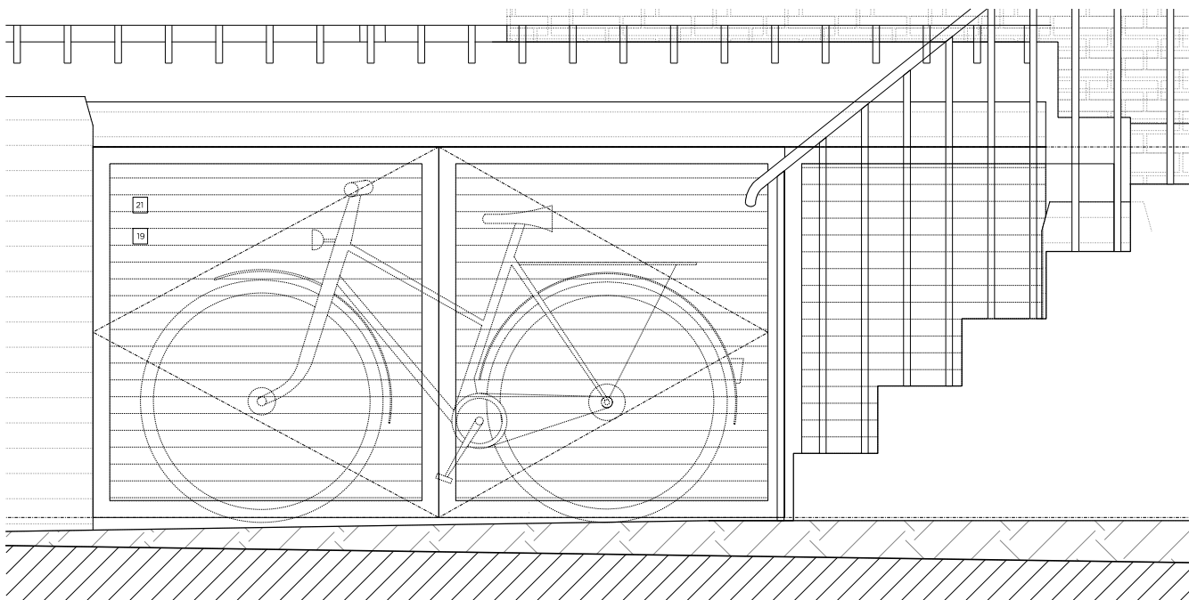
P_03 03 Cycle Store Elevation 1:20
