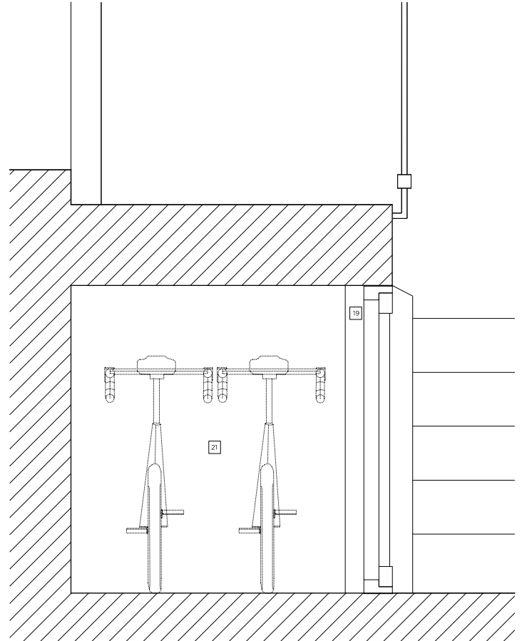
P_03 02 Cycle Store Section A-A 1:20
