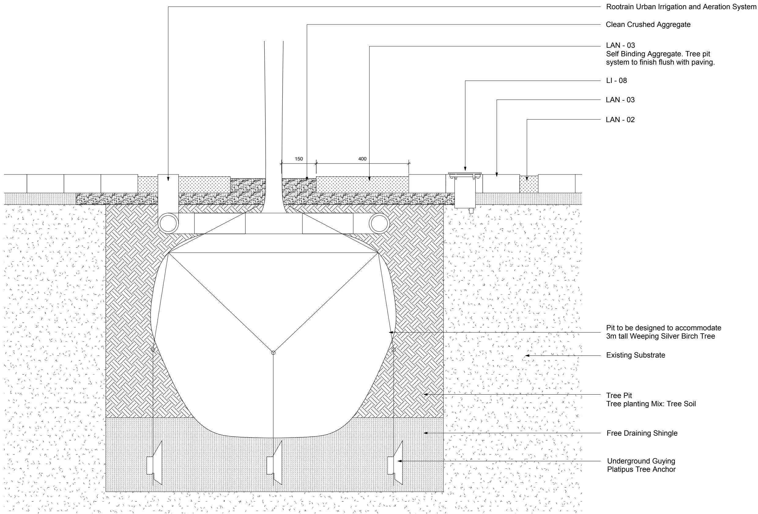
de 07 Detail Of Tree Pitt - Weeping Birch 1:5 @ A1, 1:10 @ A3
