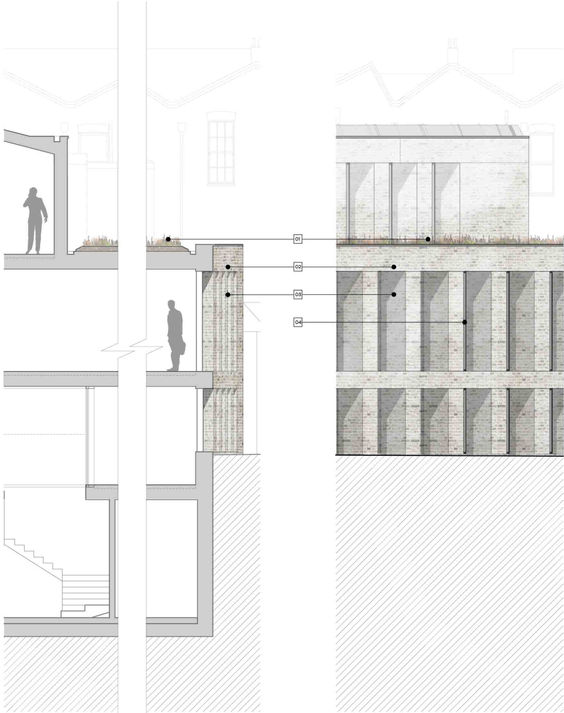
P_40 03 Section B-B 1:50
