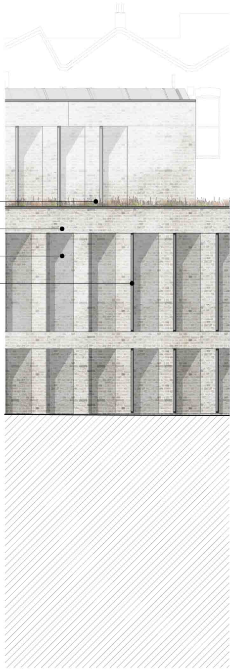
P_40 02 South East Elevation 1:50
