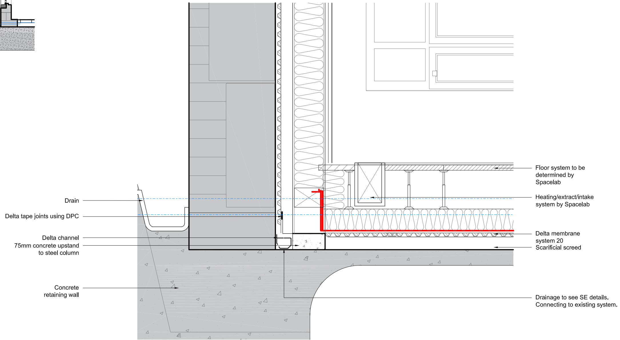
Detail 2: 1:10
