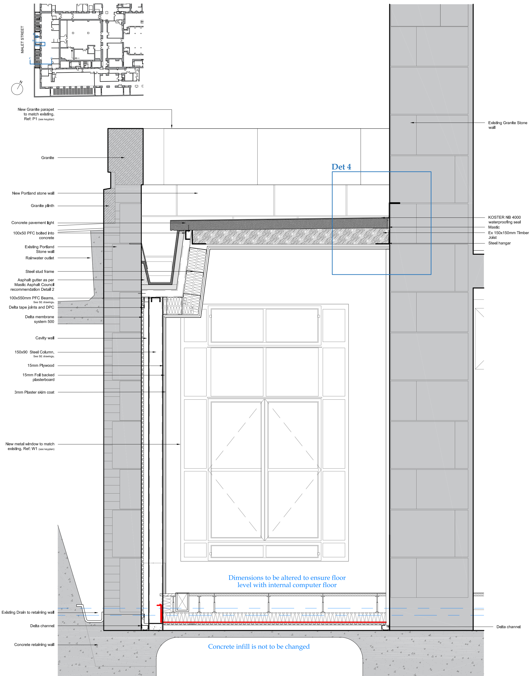
Section CC 1:20
