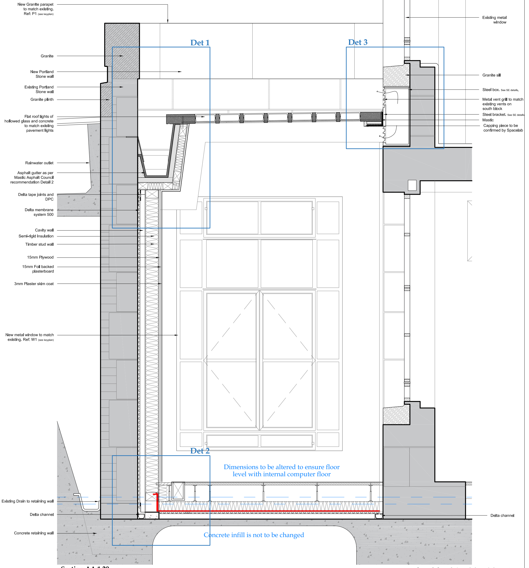
Section AA 1:20
