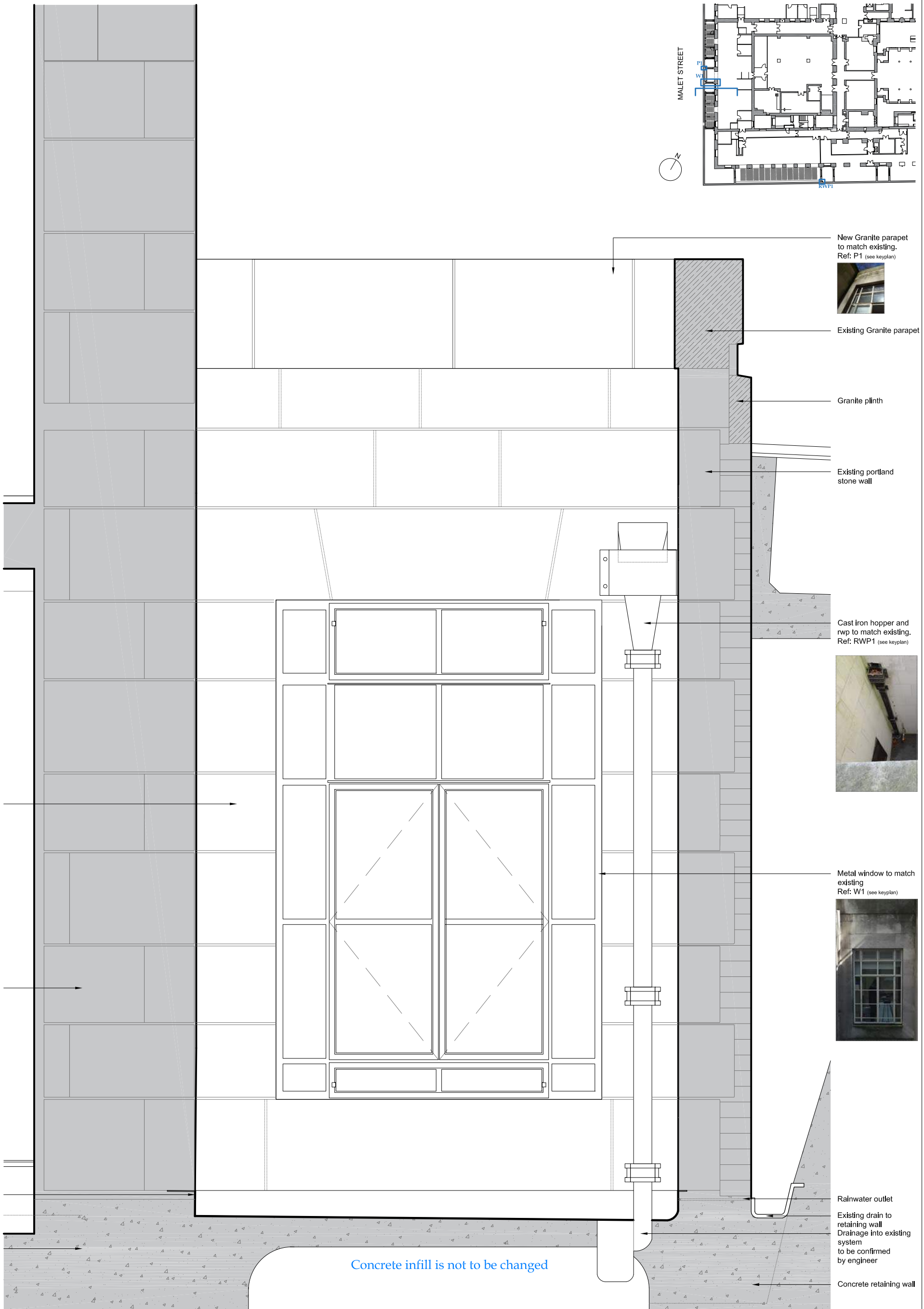
North Elevation 1:20
