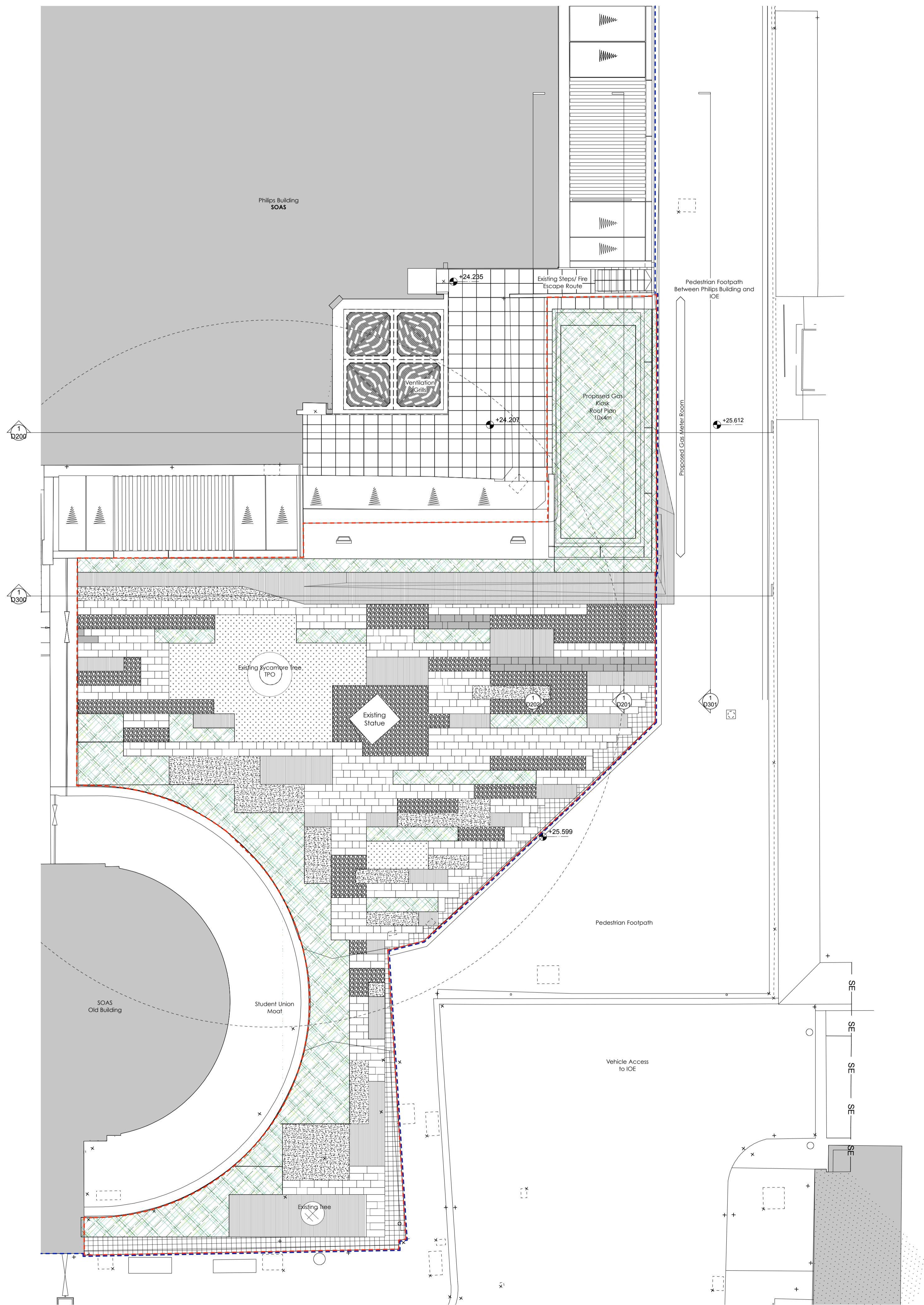
1 Proposed Site Masterplan Scale: 1:100
