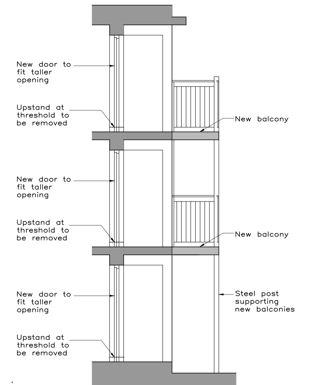
SECTION
