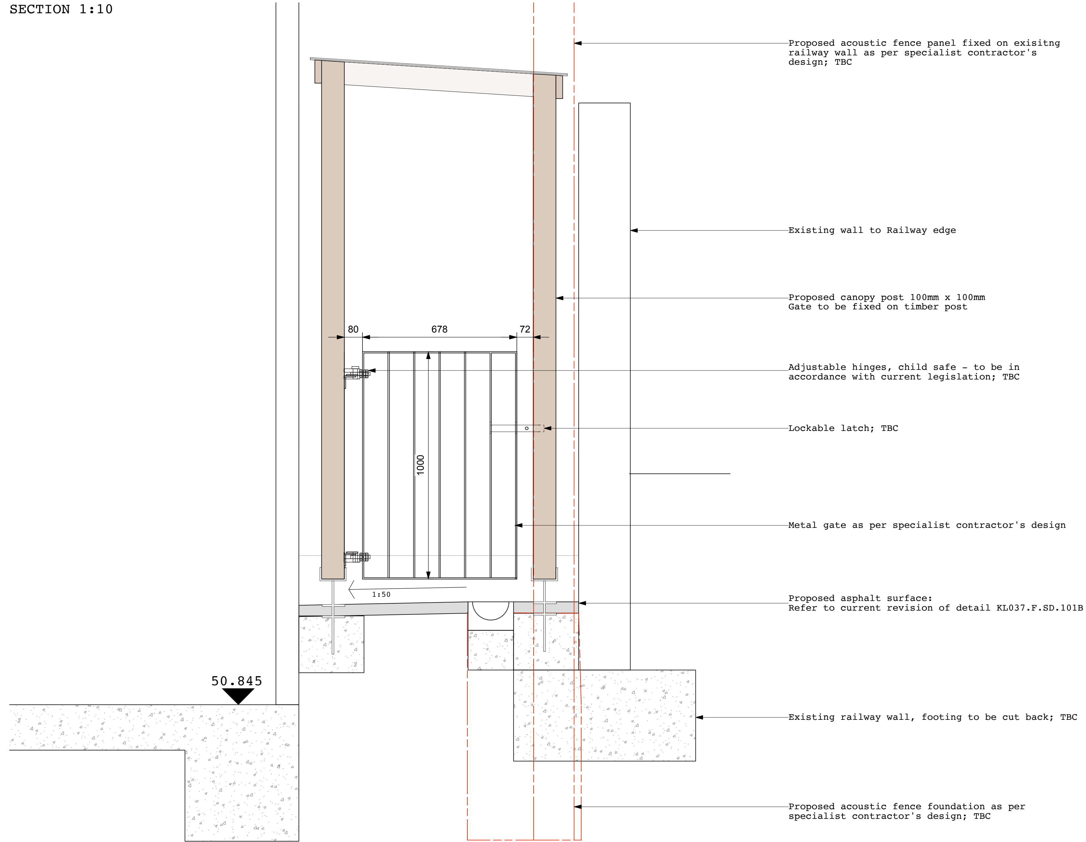
SECTION 1:10
