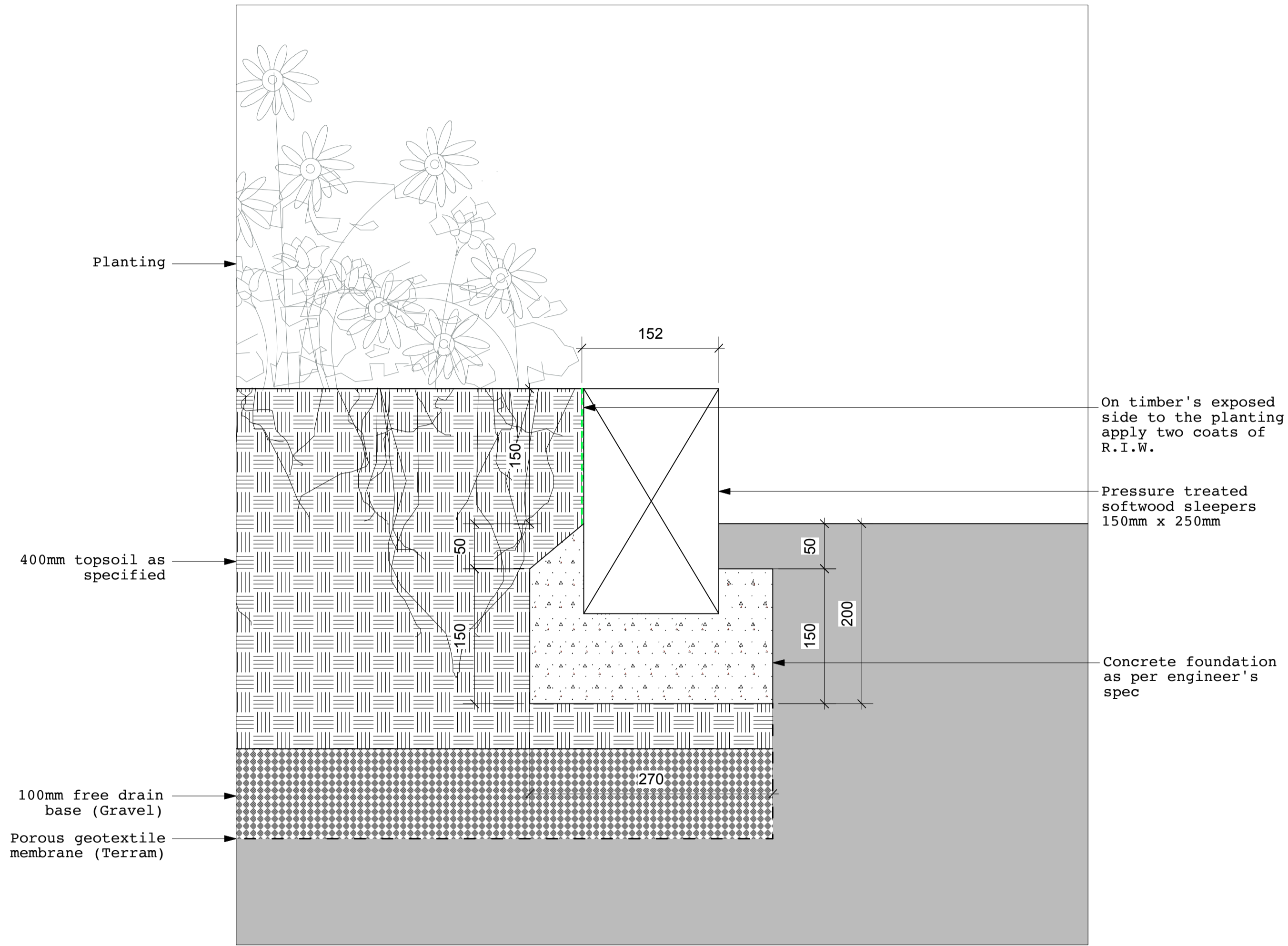
DETAIL 302A
