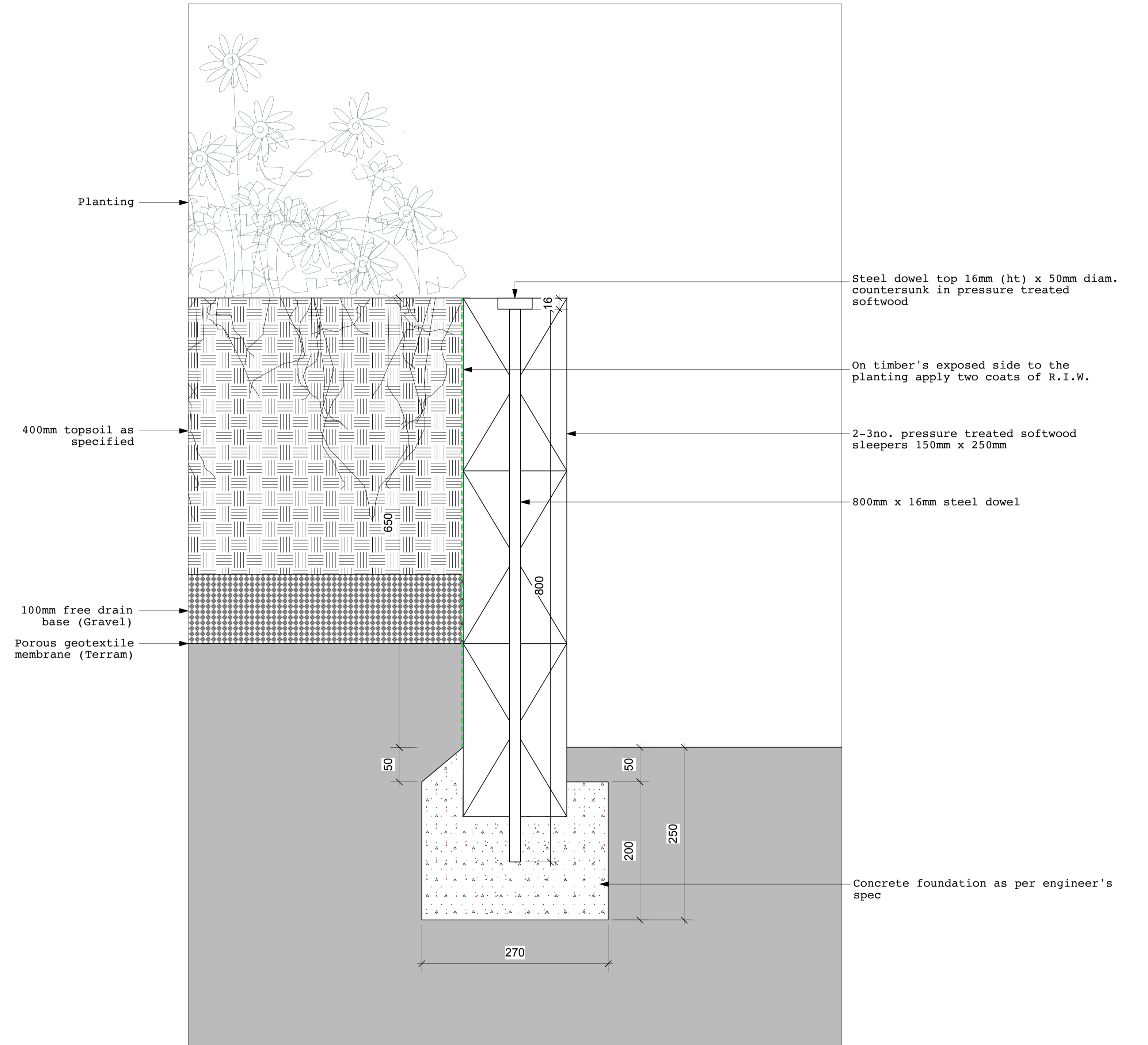
DETAIL 302B
