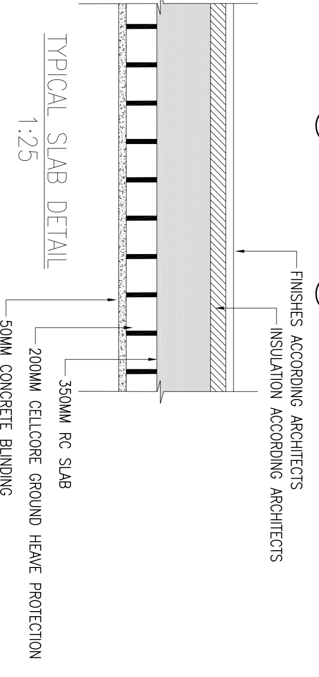
TYPICAL SLAB DETAIL 1:25
