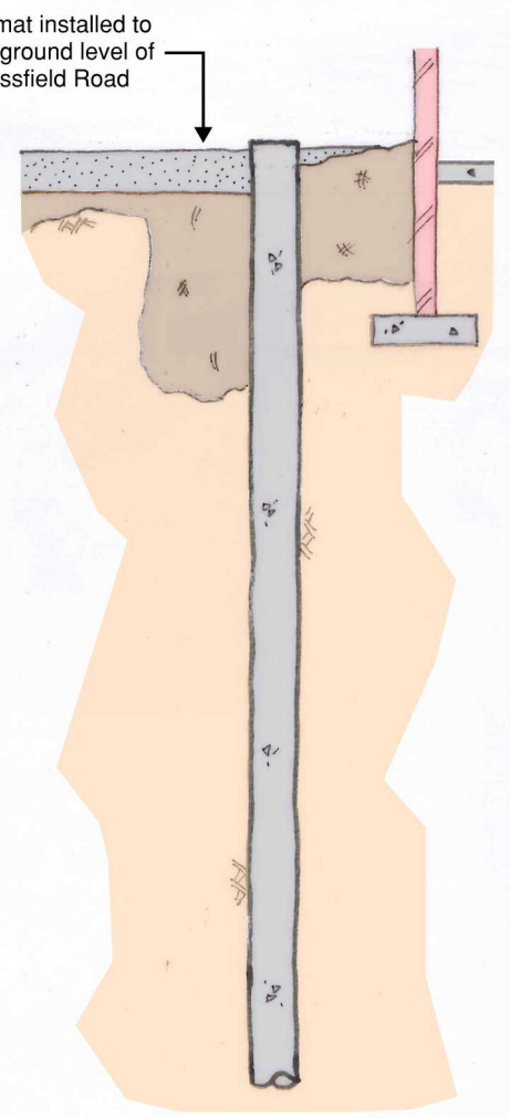
Stage 3: Piling
