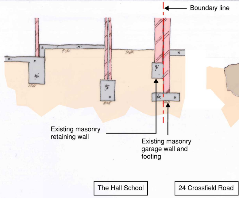
Stage 1: Existing
