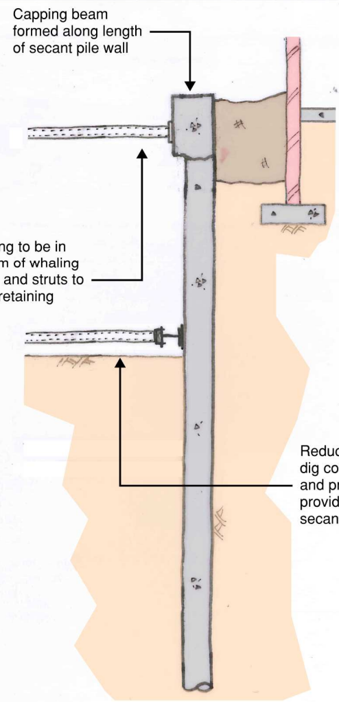
Stage 4: Reduced Level Dig
