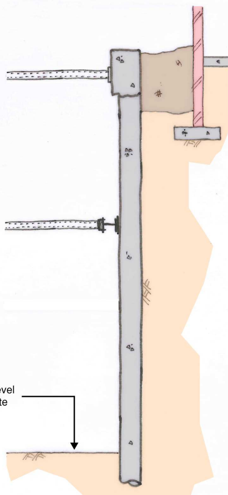
Stage 5: Complete Reduced Level Dig
