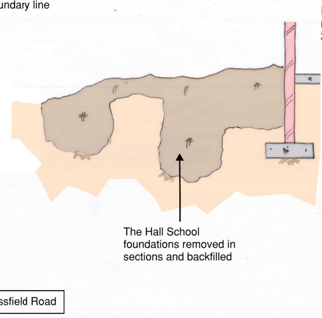
Stage 2: Demolition
