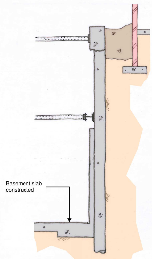
Stage 6: Commence Basement Construction
