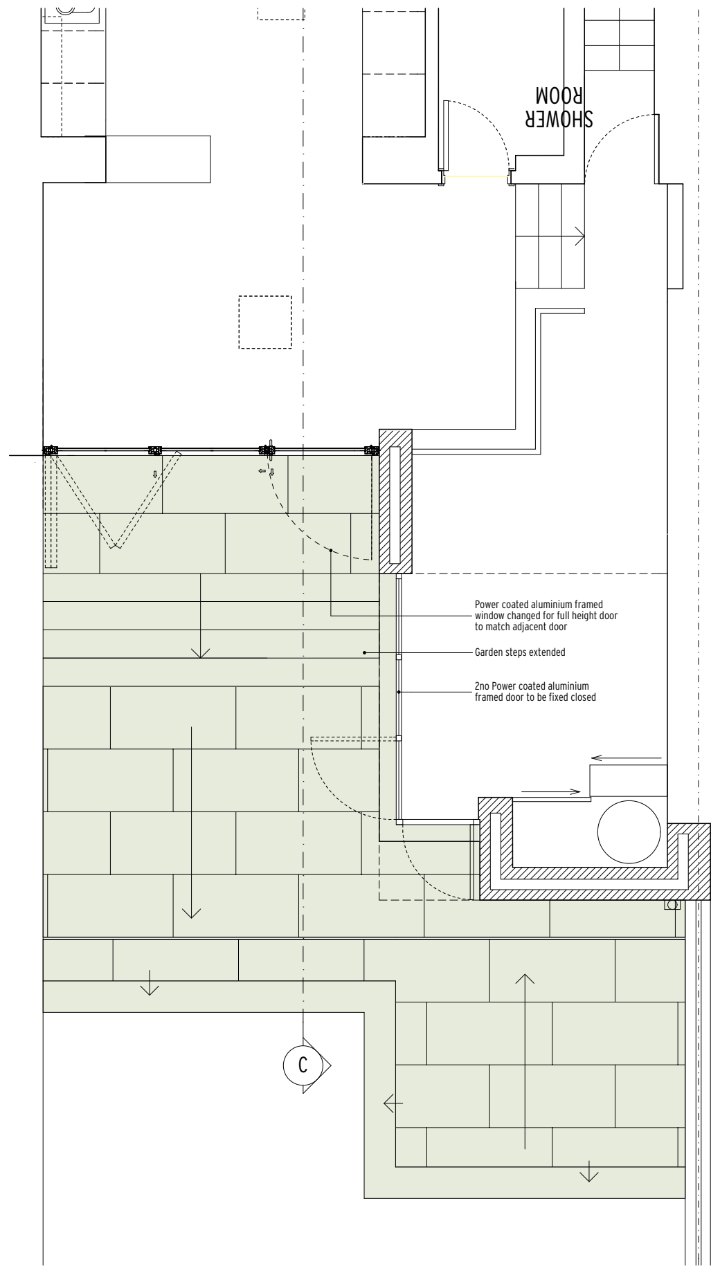
PROPOSED LOWER GROUND FLOOR PART PLAN @ 1:25 A1
