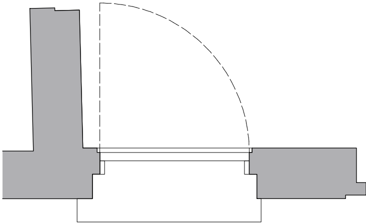
EXISTING DOOR PLAN 1:20 AT A3
