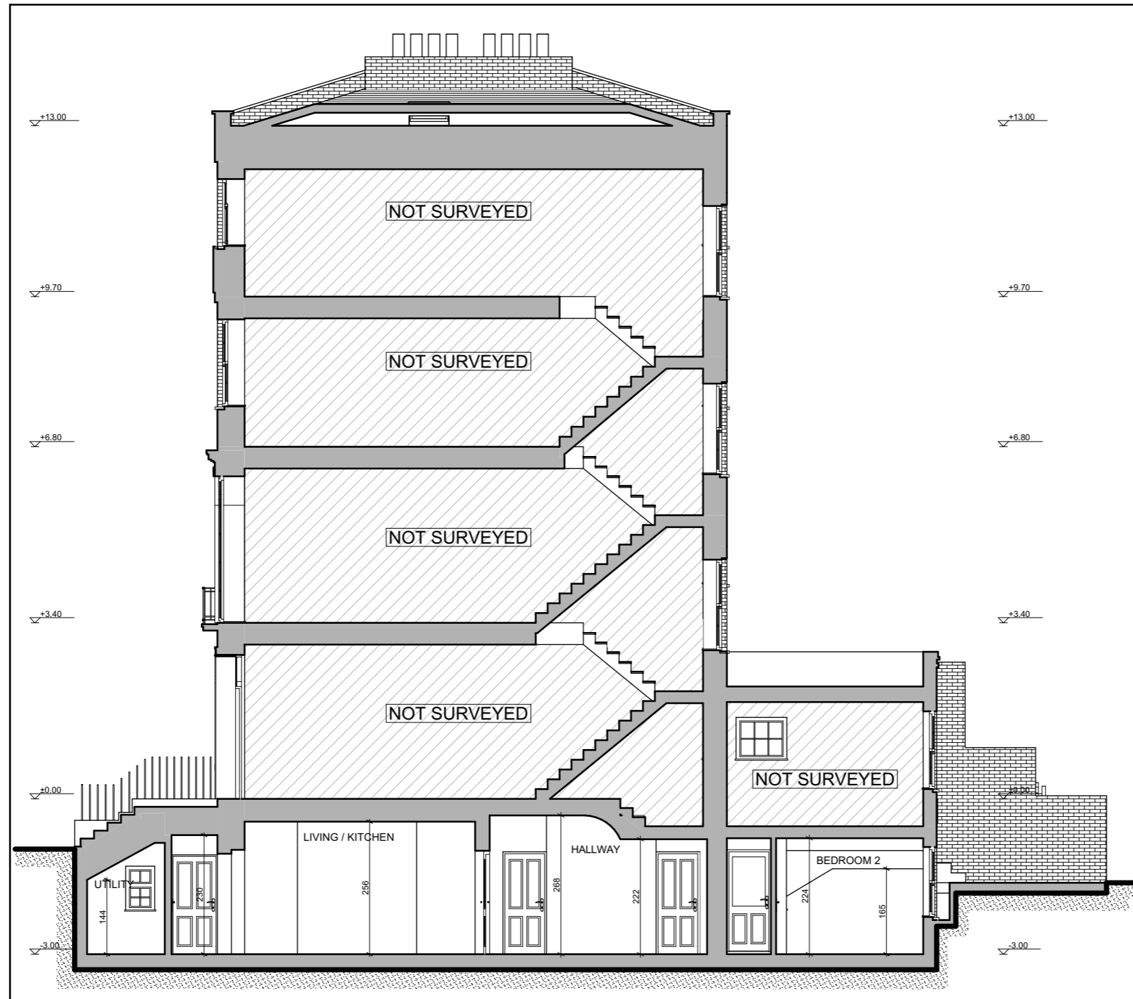
SECTION CC - PROPOSED
