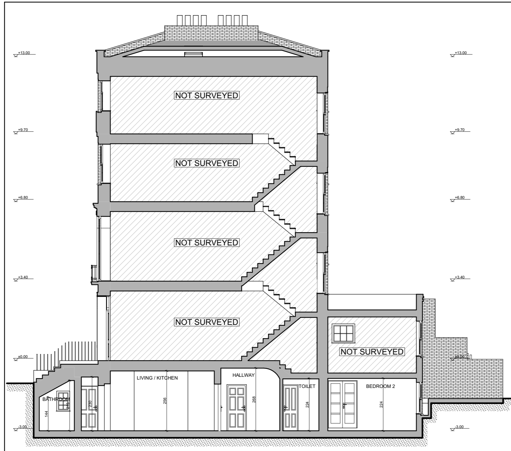
SECTION CC - EXISTING
