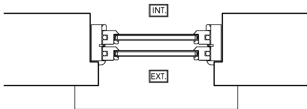
↑ B-B SECTION
