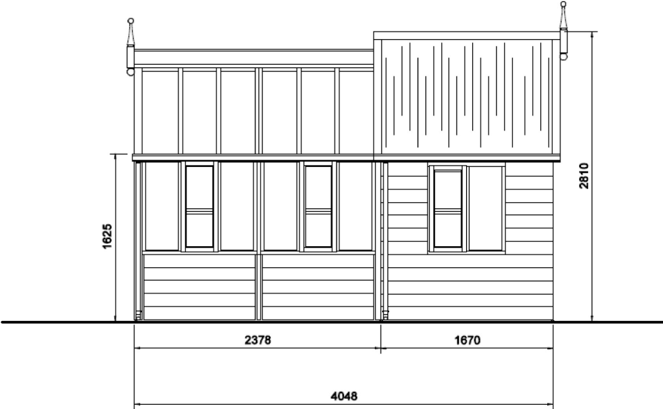
Side elevation
