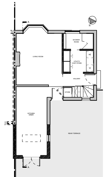
REFERENCE PLAN PROPOSED GROUND SCALE 1:200
