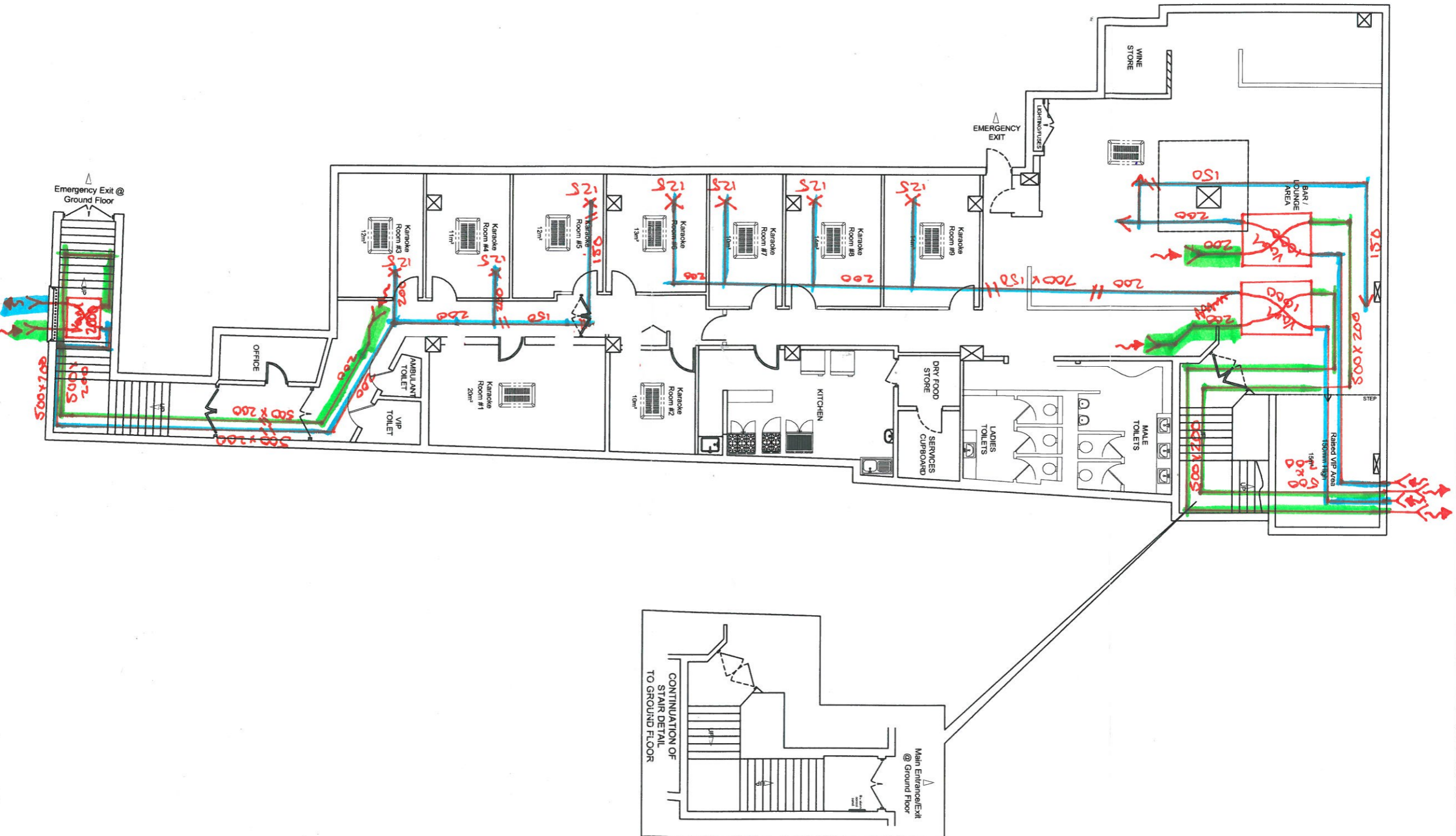
Existing Ground Floor and Basement Plan Plan @ 1:100
