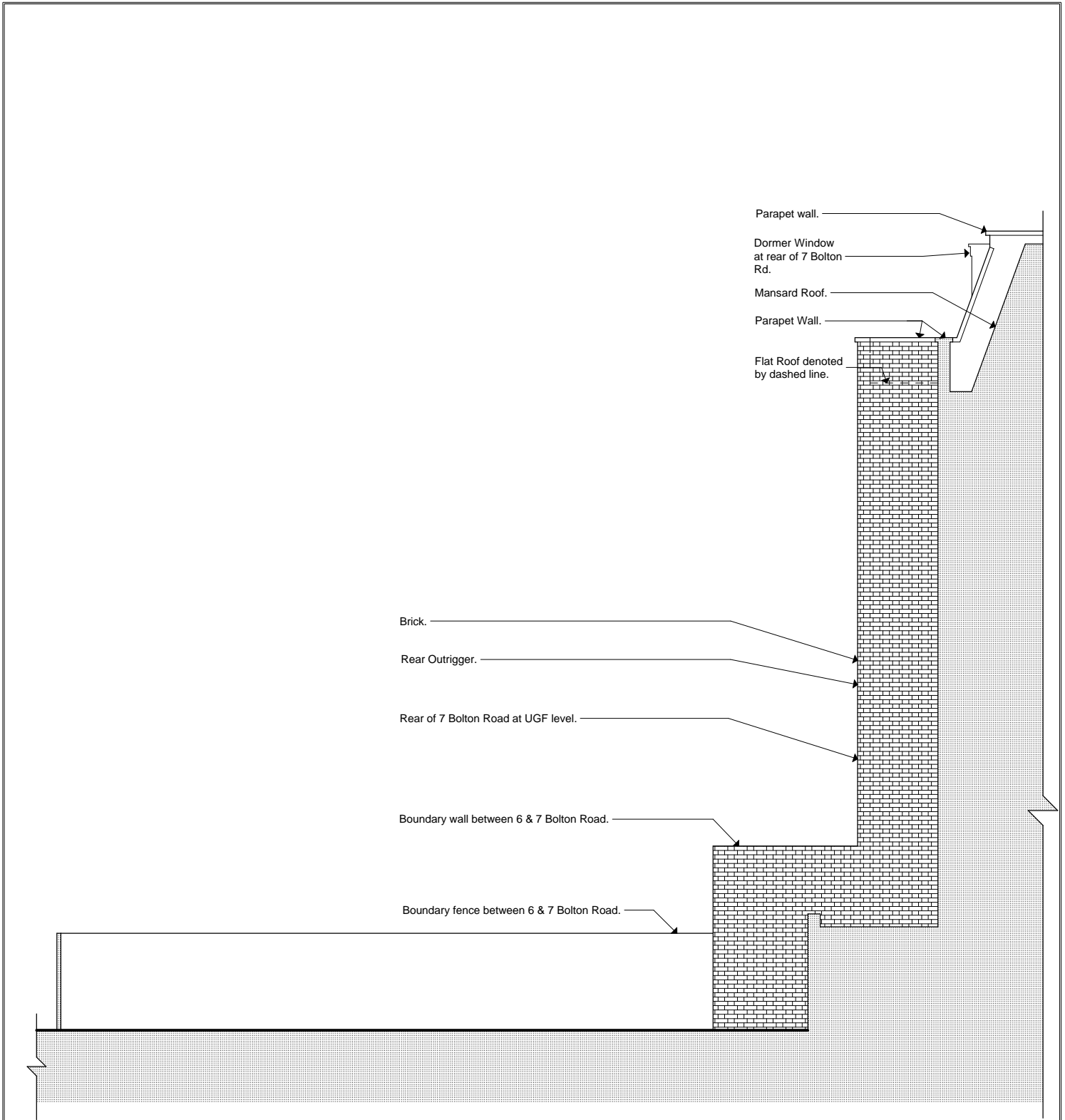
Existing East Elevation (taken through 6 Bolton Rd)
