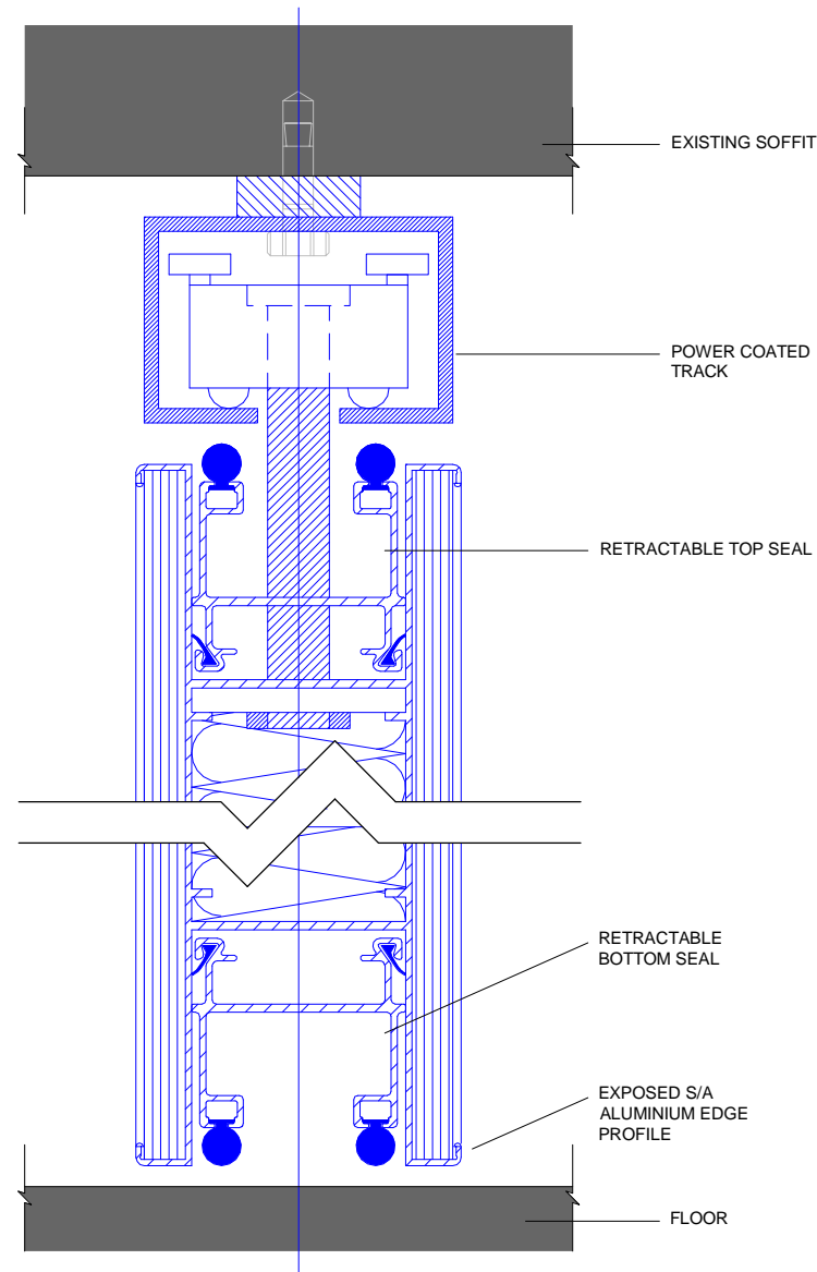
(A) Head and base detail of proposed movable partition 1:2
