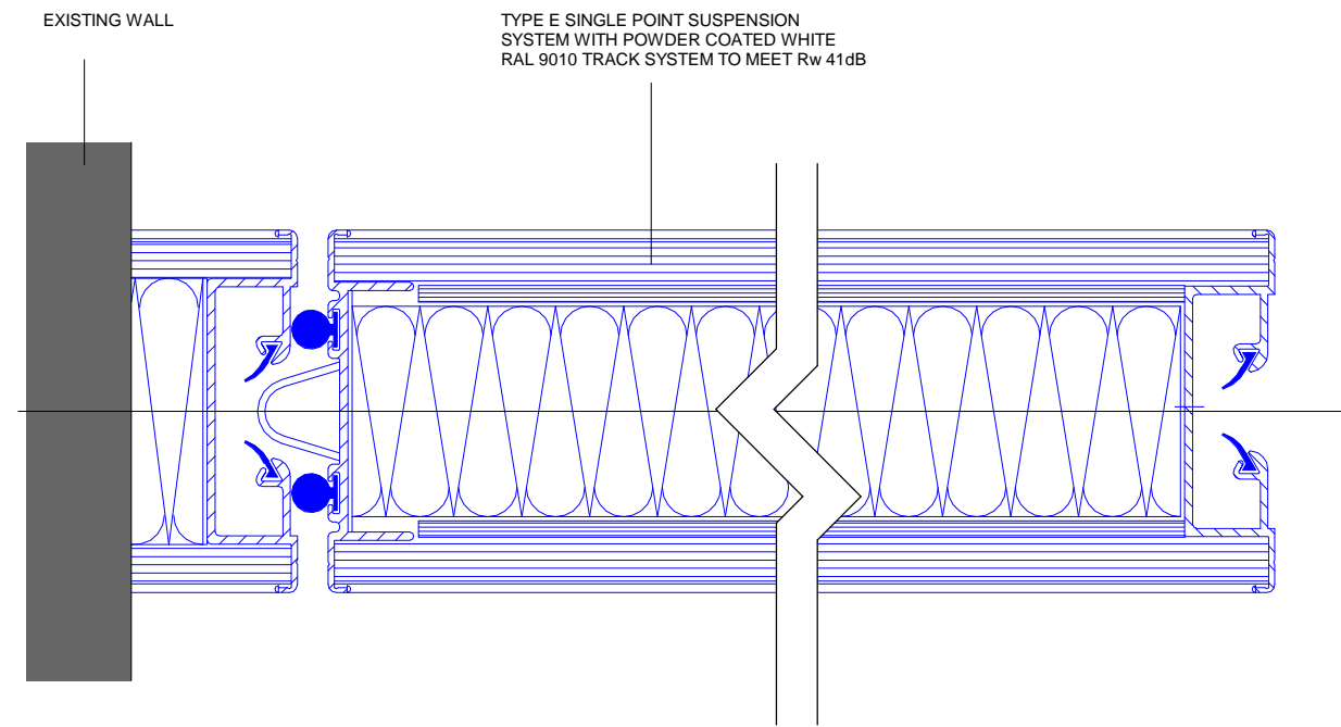
(B) Plan detail through wall junction 1:2
