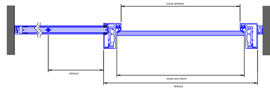
Ⓐ Plan Detail through Glazed Door 1 : 5
