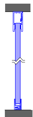
Ⓑ Head and Base Detail through Glazed Partition 1 : 5
