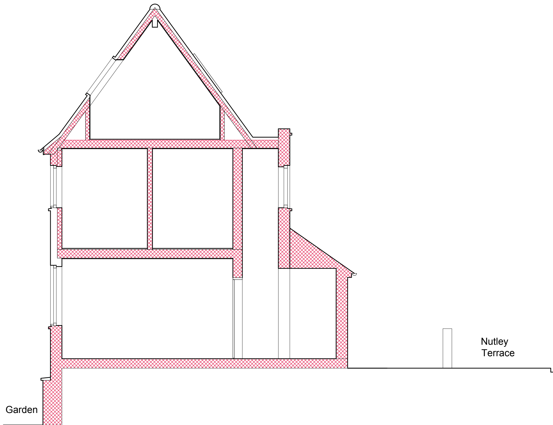
Existing Cross Section A-A
