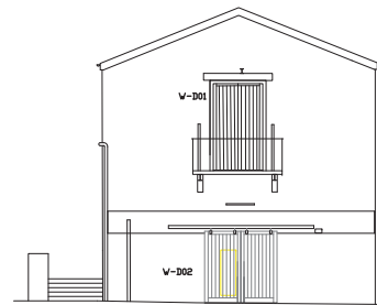
Elevation CC Scale 1:100
