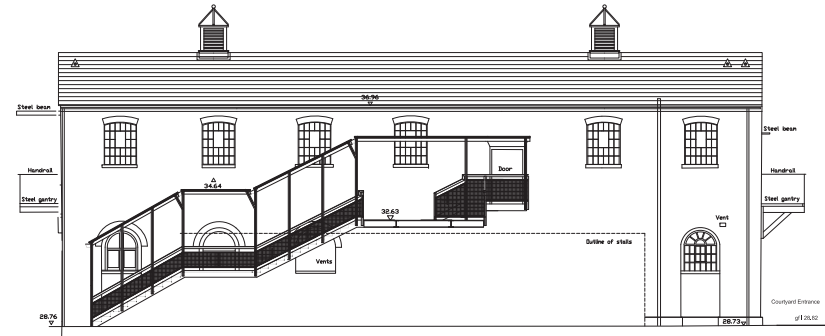
Elevation BB Scale 1:100
