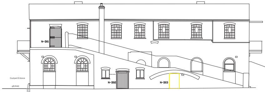
Elevation AA Scale 1:100
