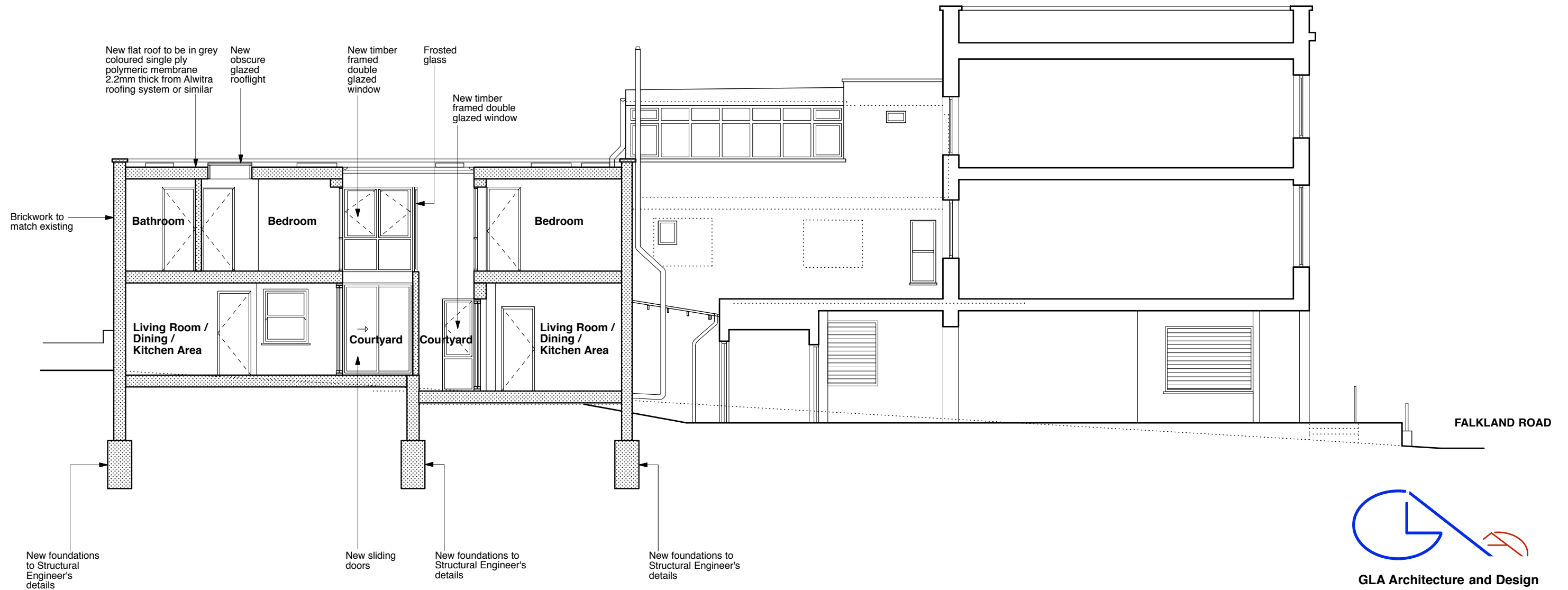
PROPOSED SECTION AA scale 1:100
