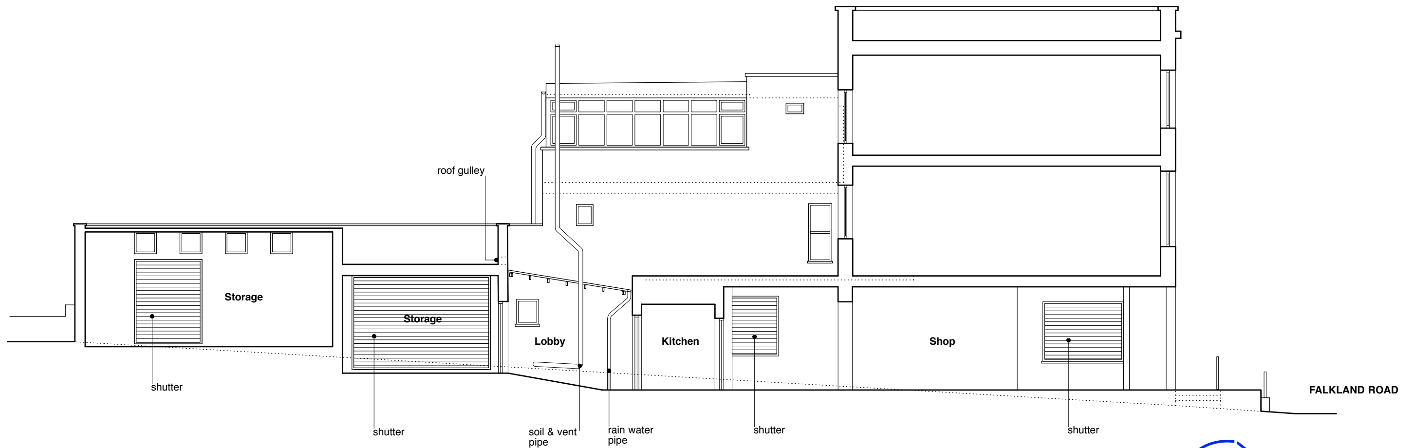
EXISTING SECTION AA scale 1:100
