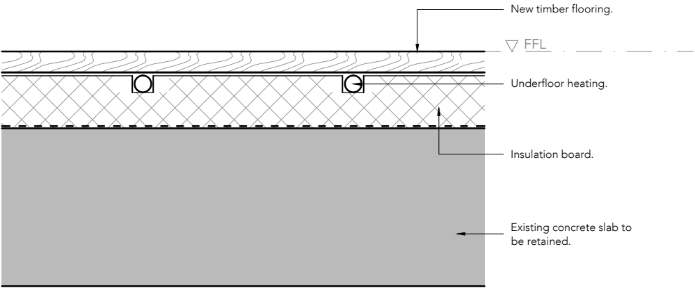
1 LOWER GROUND FLOOR SLAB BUILT UP scale 1:5
