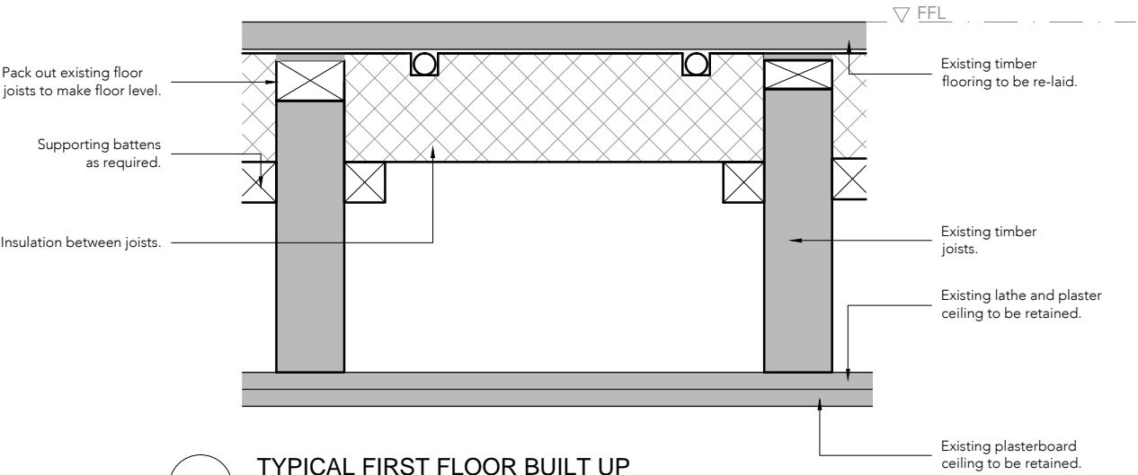
2 TYPICAL FIRST FLOOR BUILT UP scale 1:5
