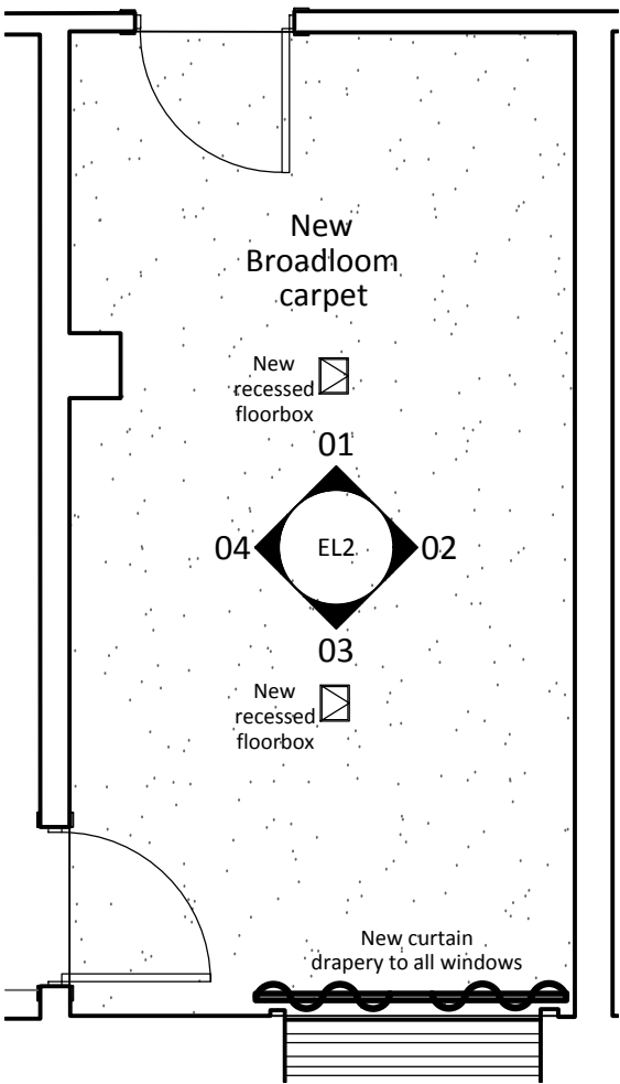
Proposed Floor layout
