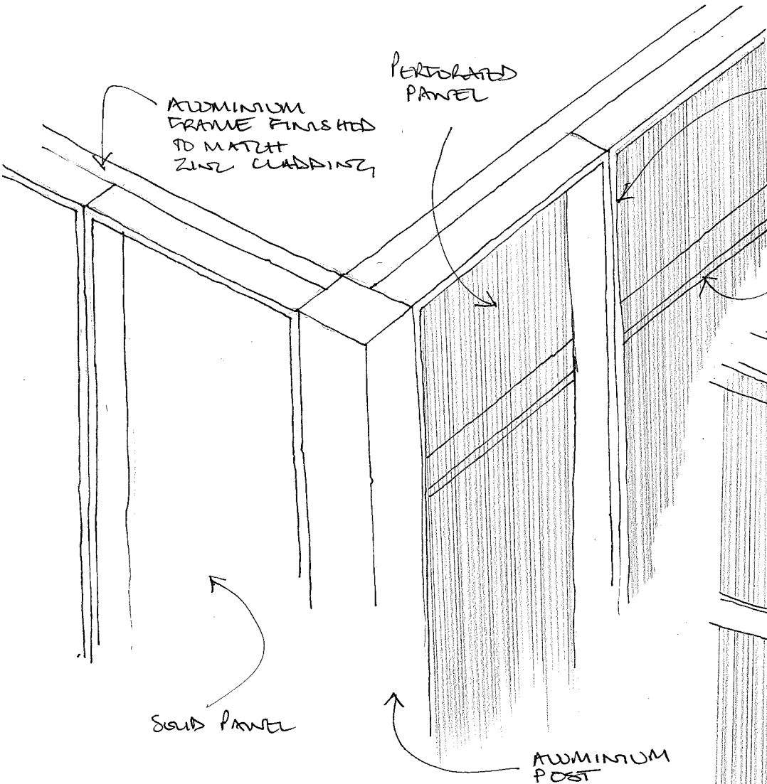
SK-01 ISOMETRIC SKETCH LOOKING AT SCREEN FROM OUTSIDE (NORTH / EAST CORNER)
