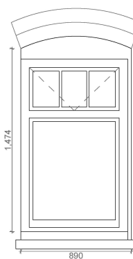
PROPOSED GROUND FLOOR WINDOW ELEVATION
