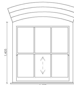
PROPOSED FIRST FLOOR WINDOW ELEVATION
