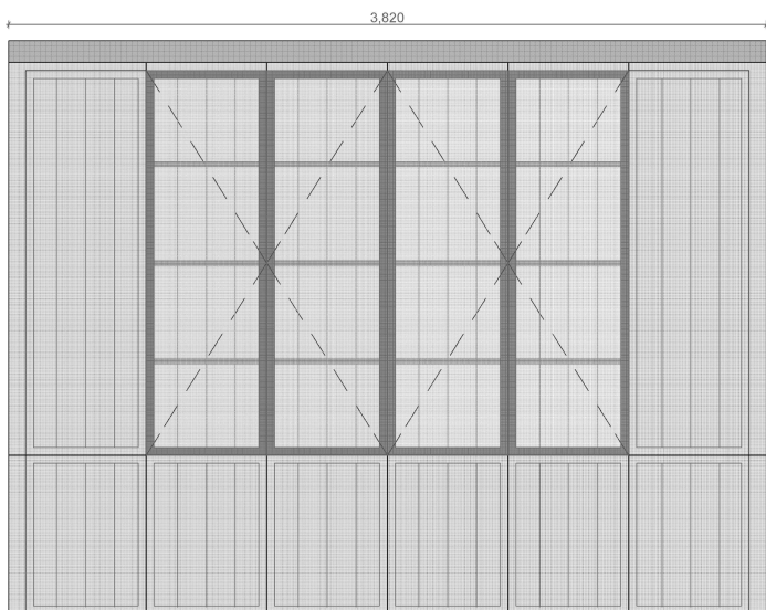
PROPOSED DOOR ELEVATION - SHUTTERS CLOSE - BEHIND GLAZING
