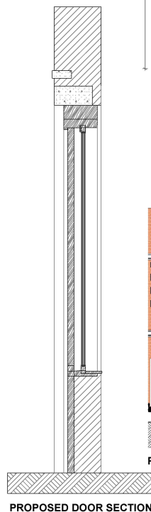
PROPOSED DOOR SECTION
