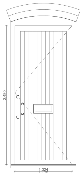
PROPOSED ENTRANCE DOOR ELEVATION
