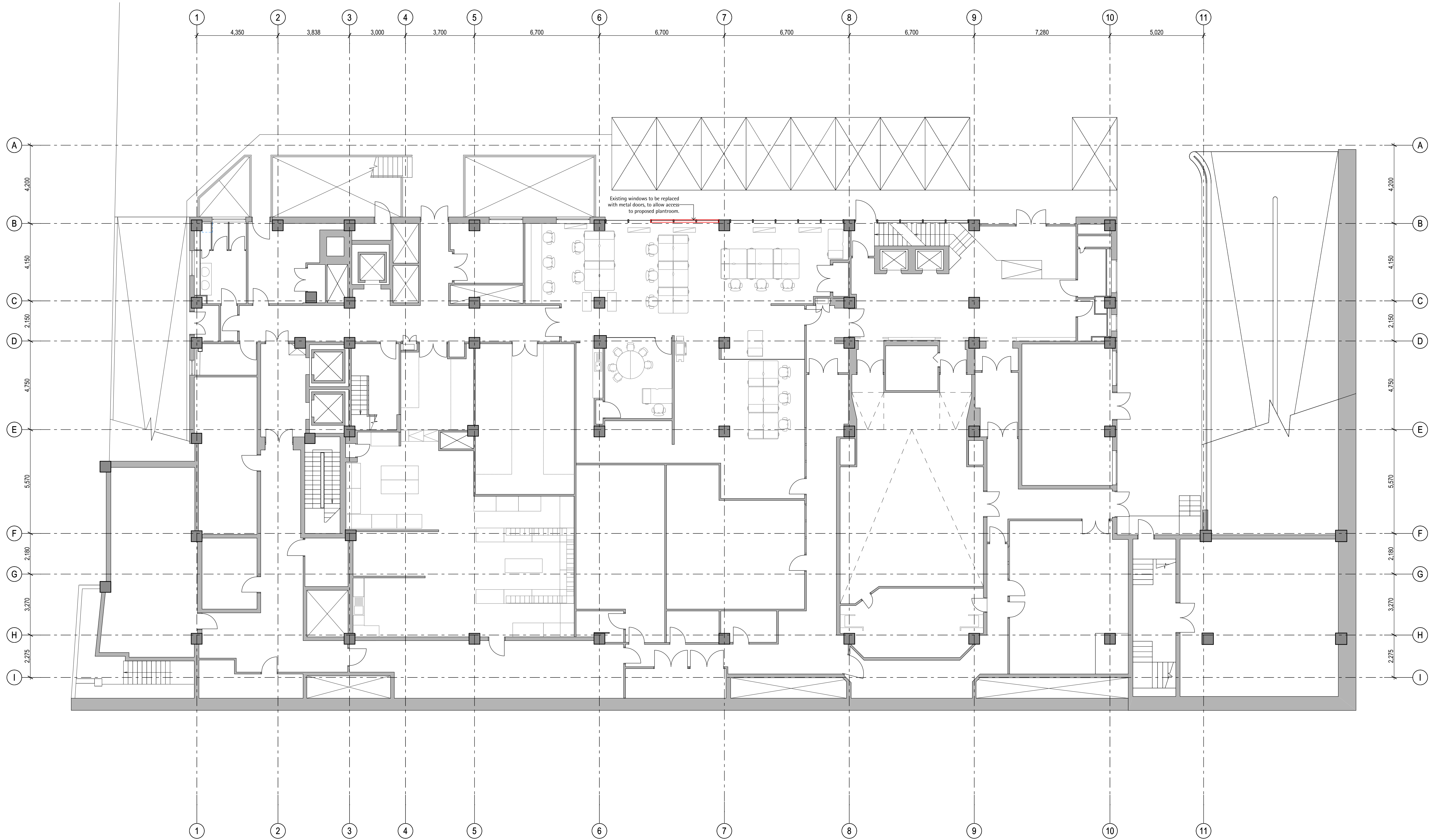
1 B1 Basement Floor - Existing SCALE 1:100
