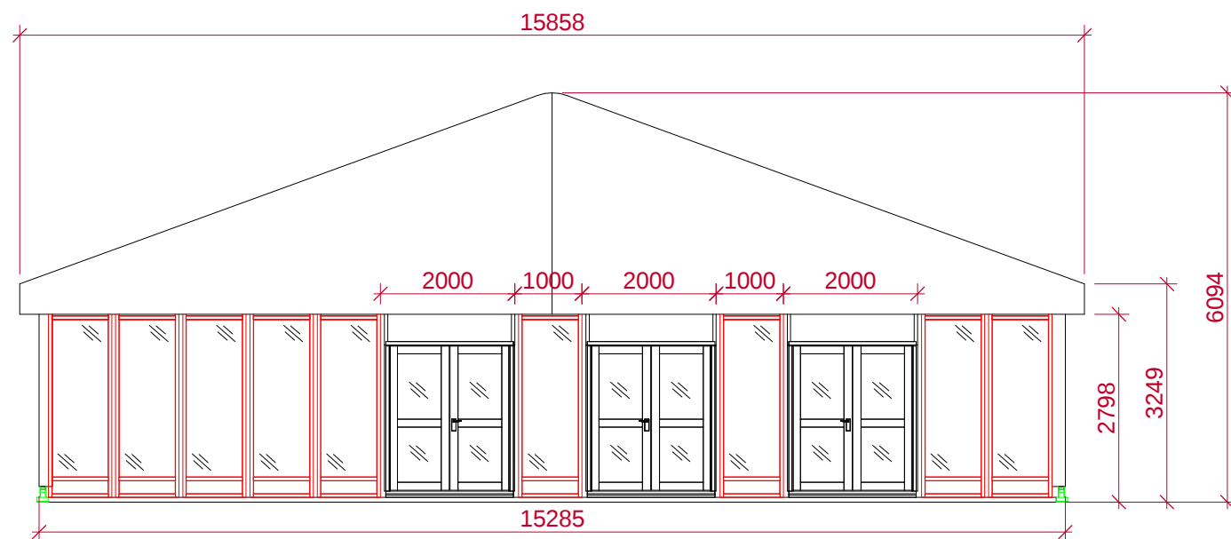
Japanese Jarden Marquee - Modified Configuration Elevation 03 - Front Entrance
