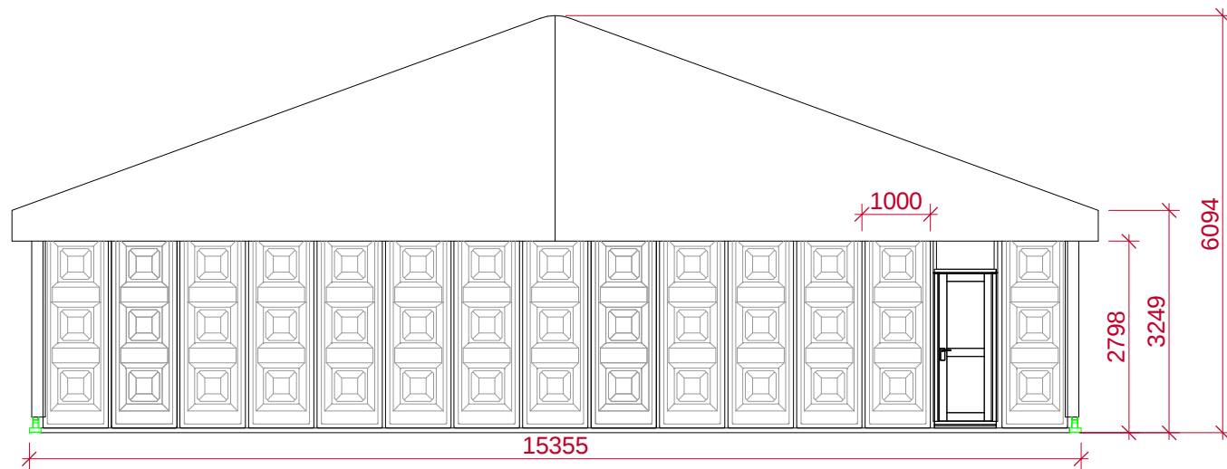
Japanese Jarden Marquee - Modified Configuration Elevation 01 - Rear
