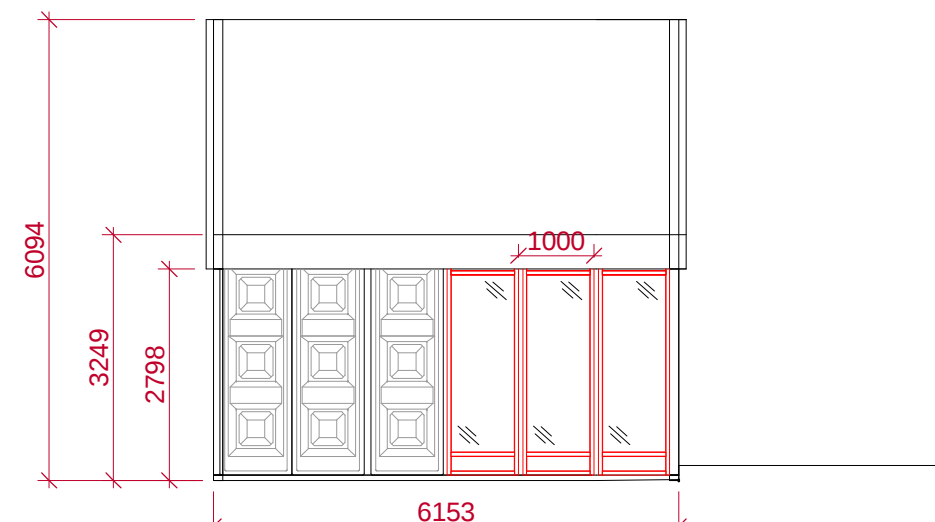
Japanese Jarden Marquee - Modified Configuration Elevation 04 - East Elevation
