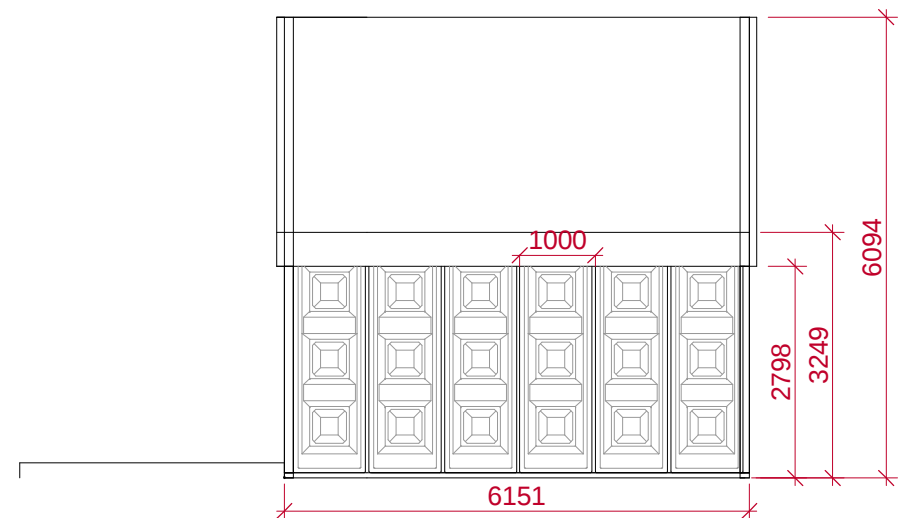
Japanese Jarden Marquee - Modified Configuration Elevation 02 - West Elevation
