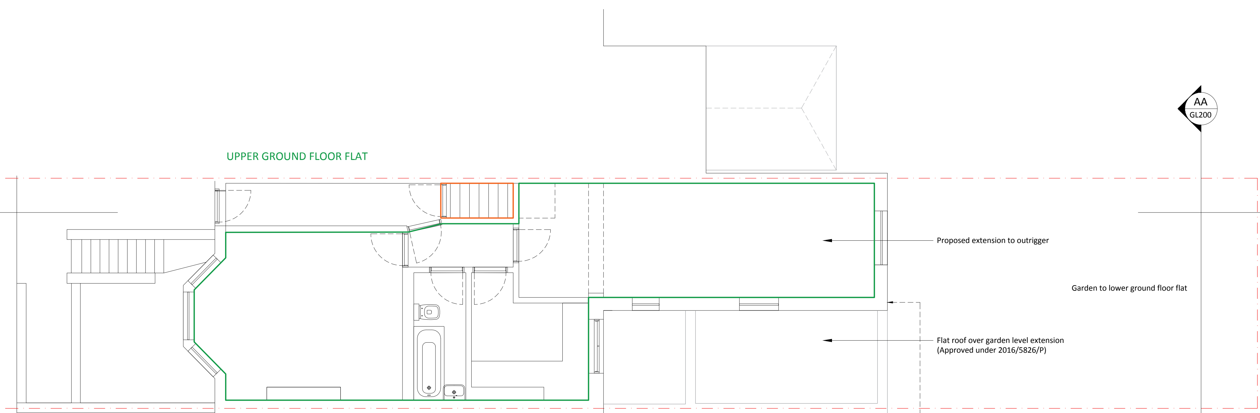
pP01 PROPOSED LAYOUT - UPPER GROUND LEVEL 0 0.5 1 2 3 1:50 at A1
