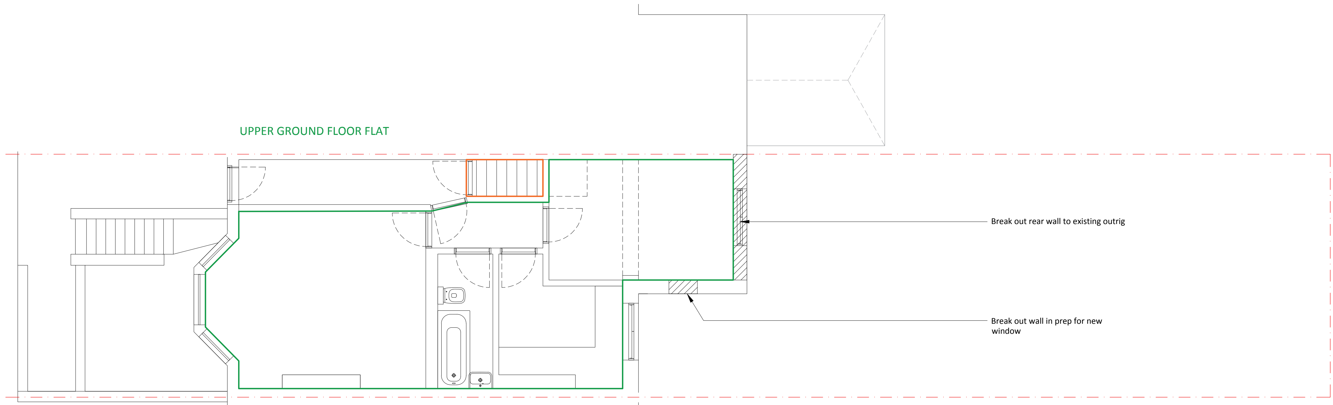
xP01 EXISTING LAYOUT - UPPER GROUND LEVEL 0 0.5 1 2 3 1:50 at A1 DEMOLITION
