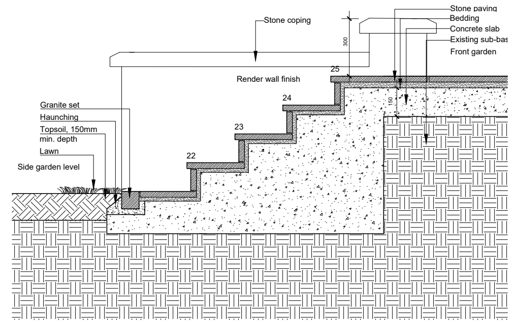
3 Detail 3: External stairs to front garden level 1:20 @ A3
