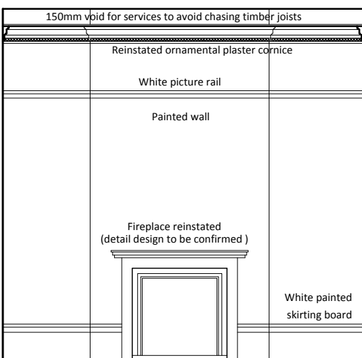
Room Elevation E Upper Ground Floor
