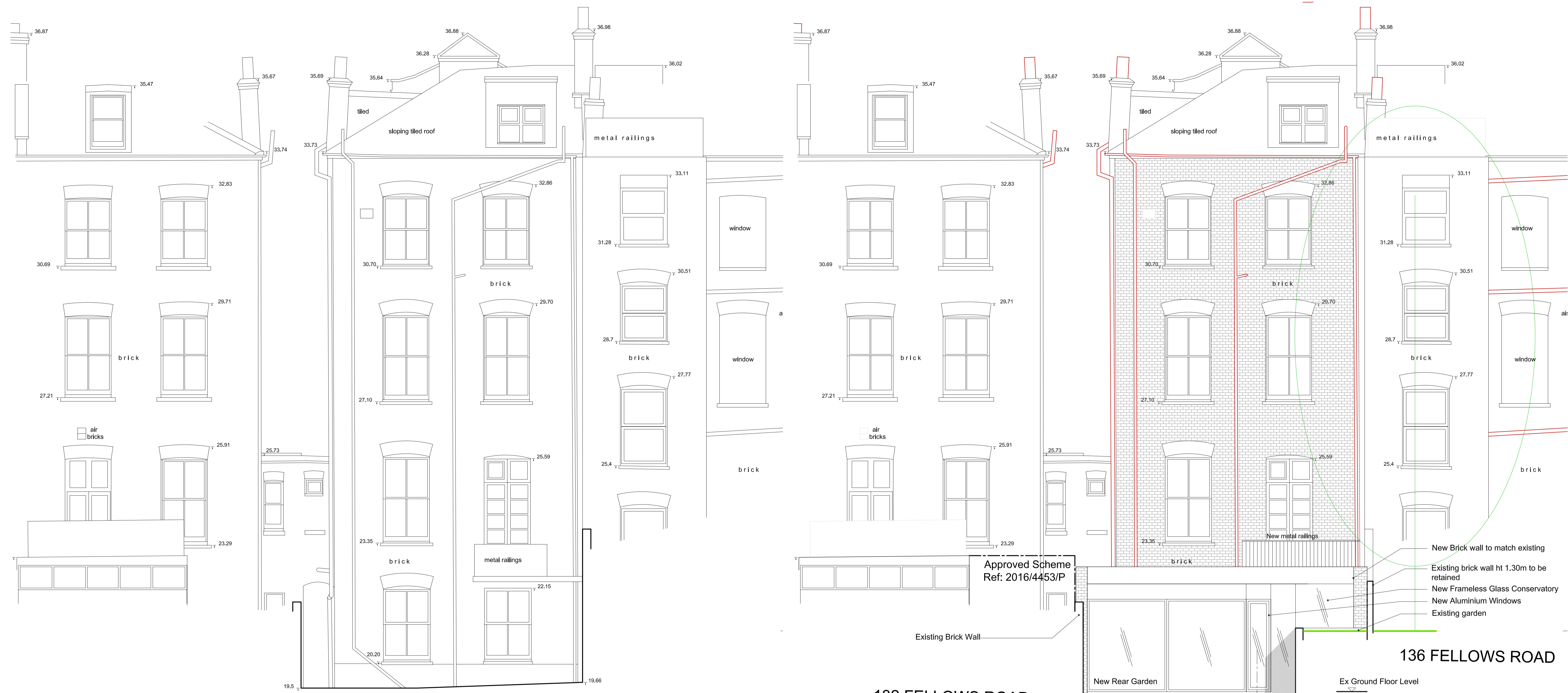
2 Proposed Rear Elevation (South)
