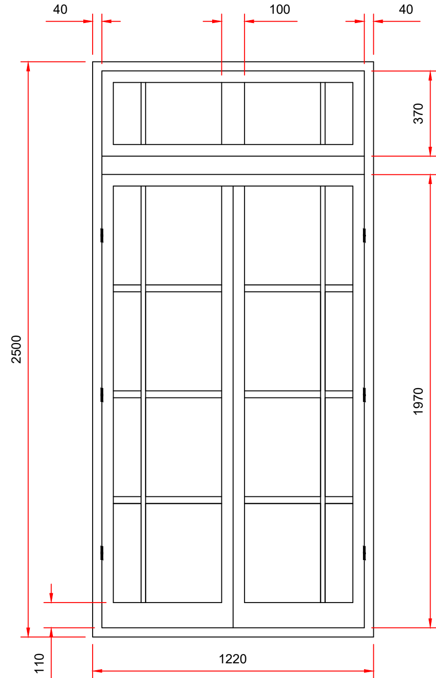
Front Elevation
