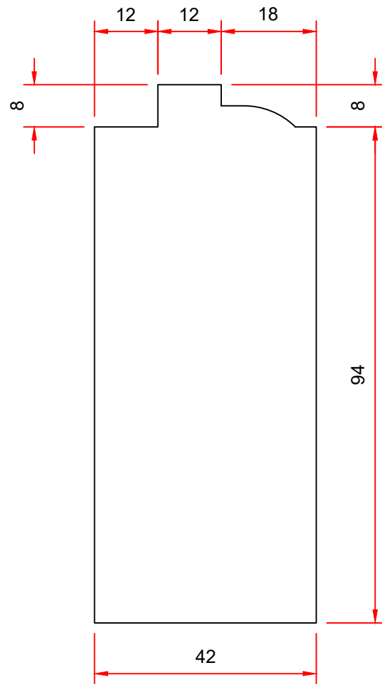
Frame Detail
