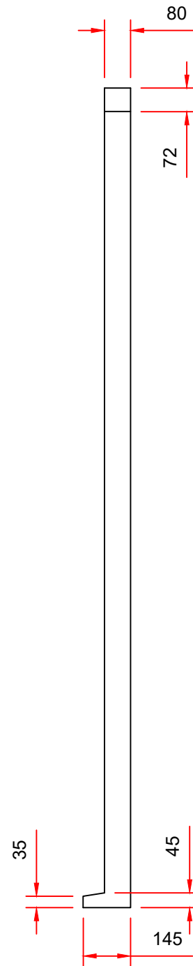
Side Elevation
