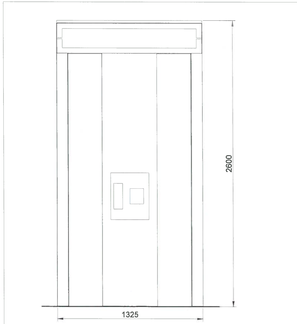
03 Front Elevation
