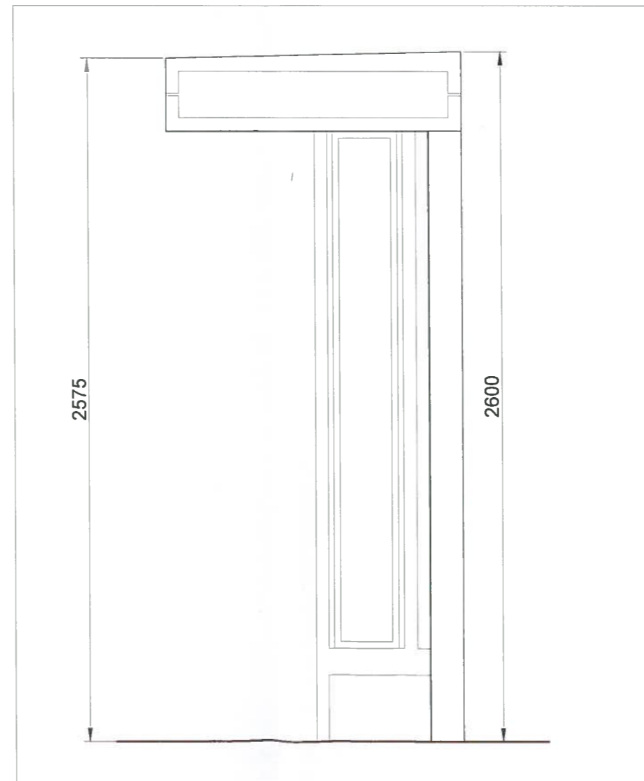
04 Side Elevation
