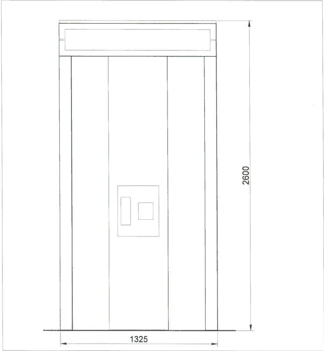
03 Front Elevation
