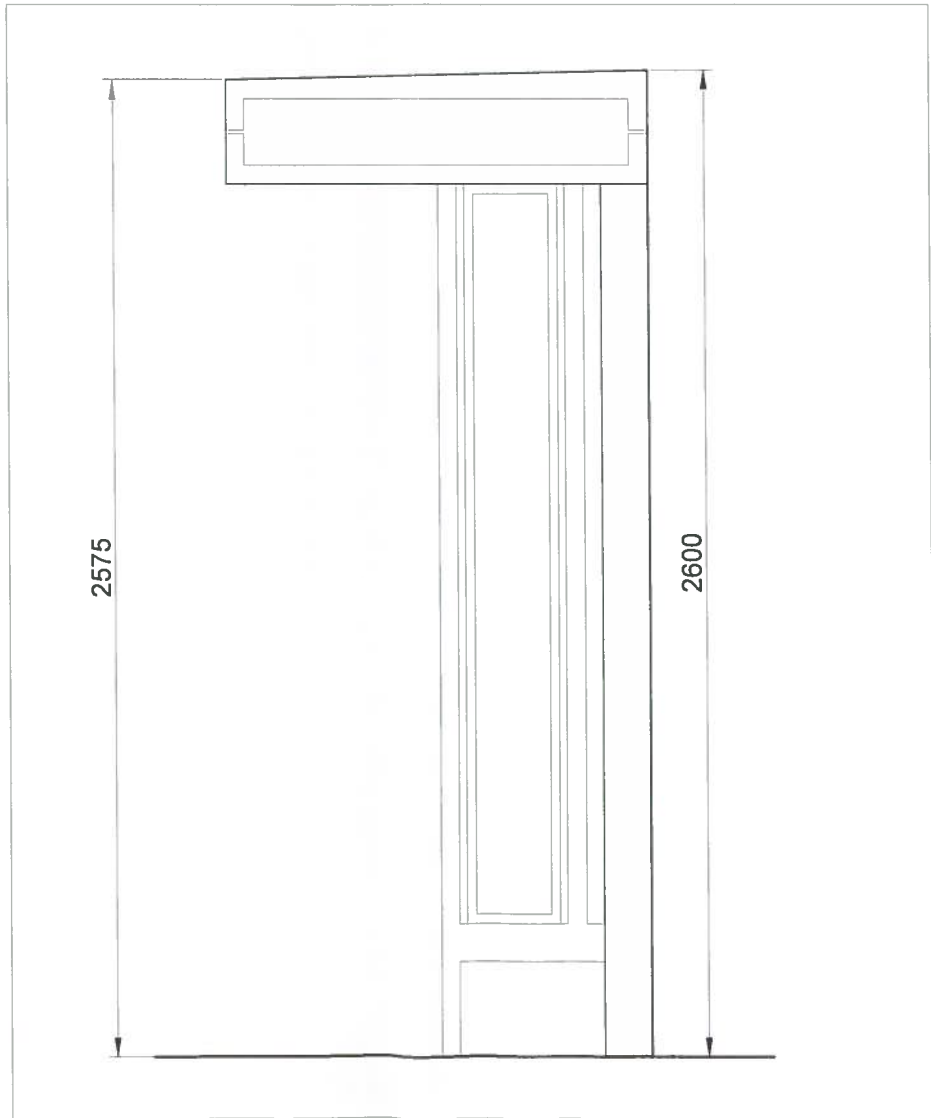
04 Side Elevation
