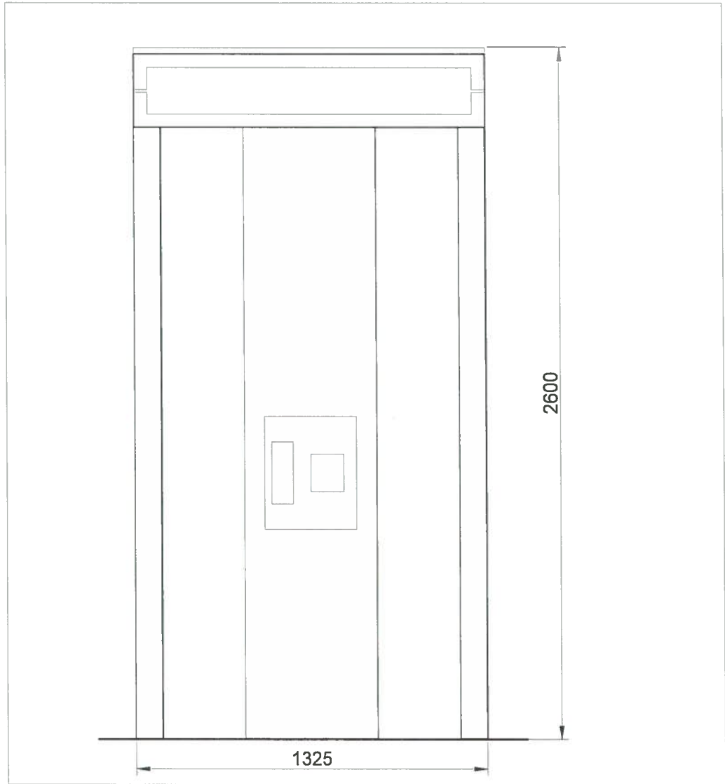
03 Front Elevation
