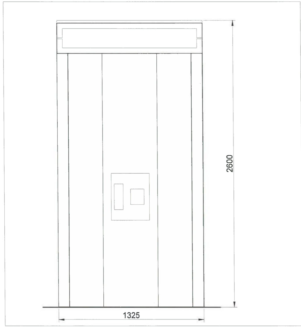
03 Front Elevation
