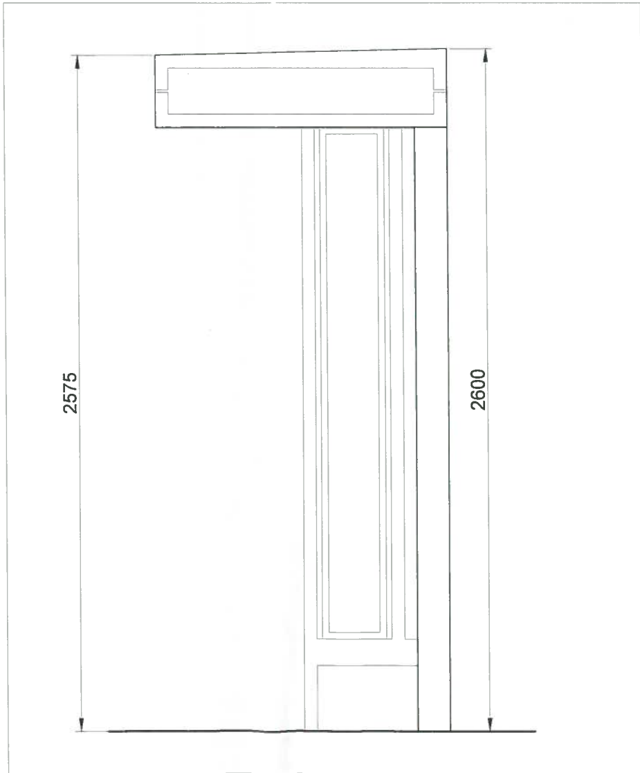
04 Side Elevation
