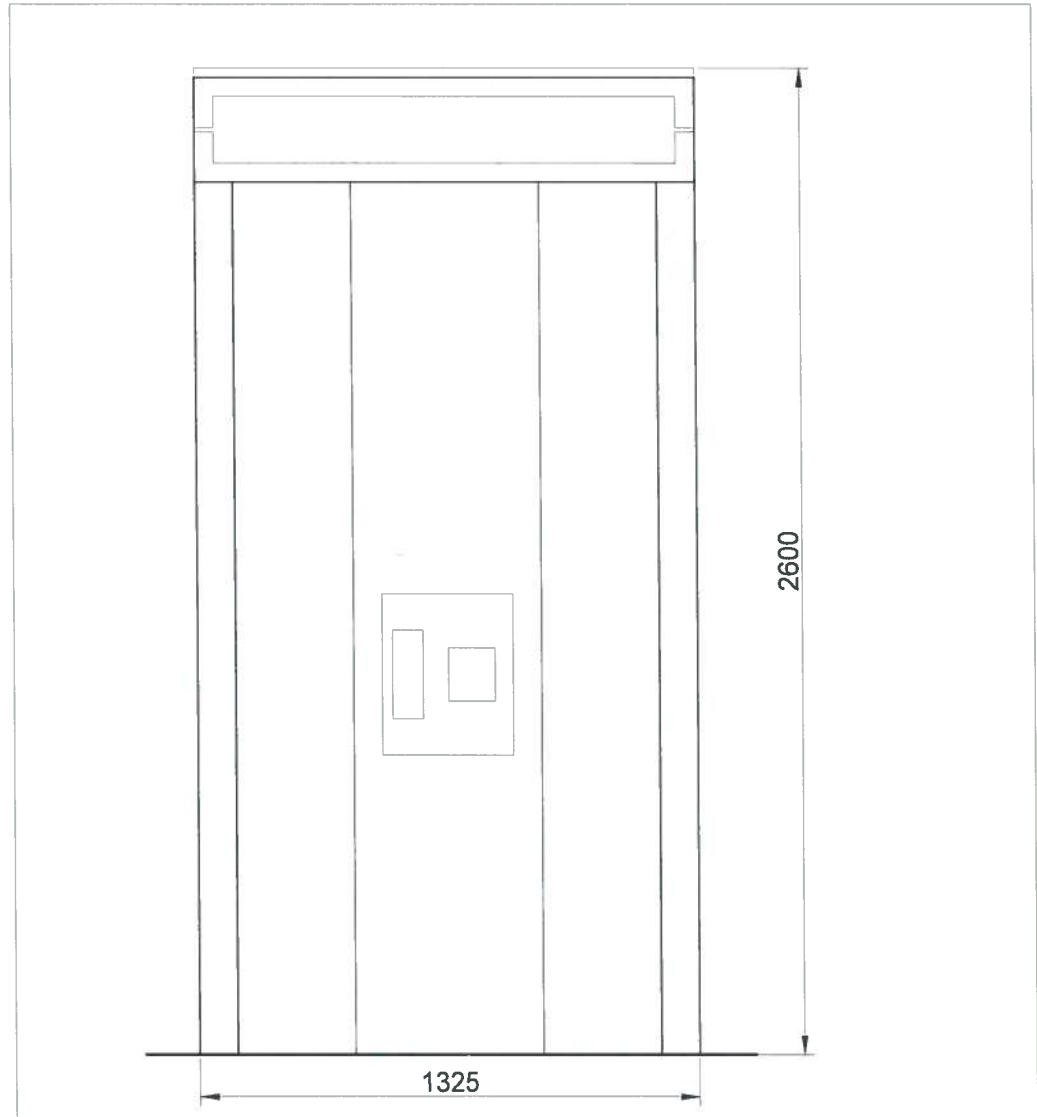
03 Front Elevation
