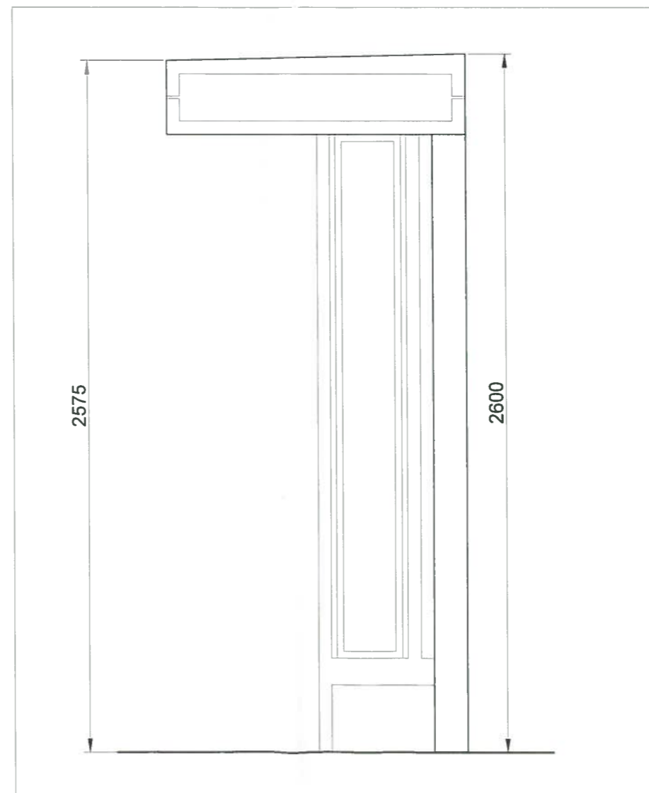
04 Side Elevation
