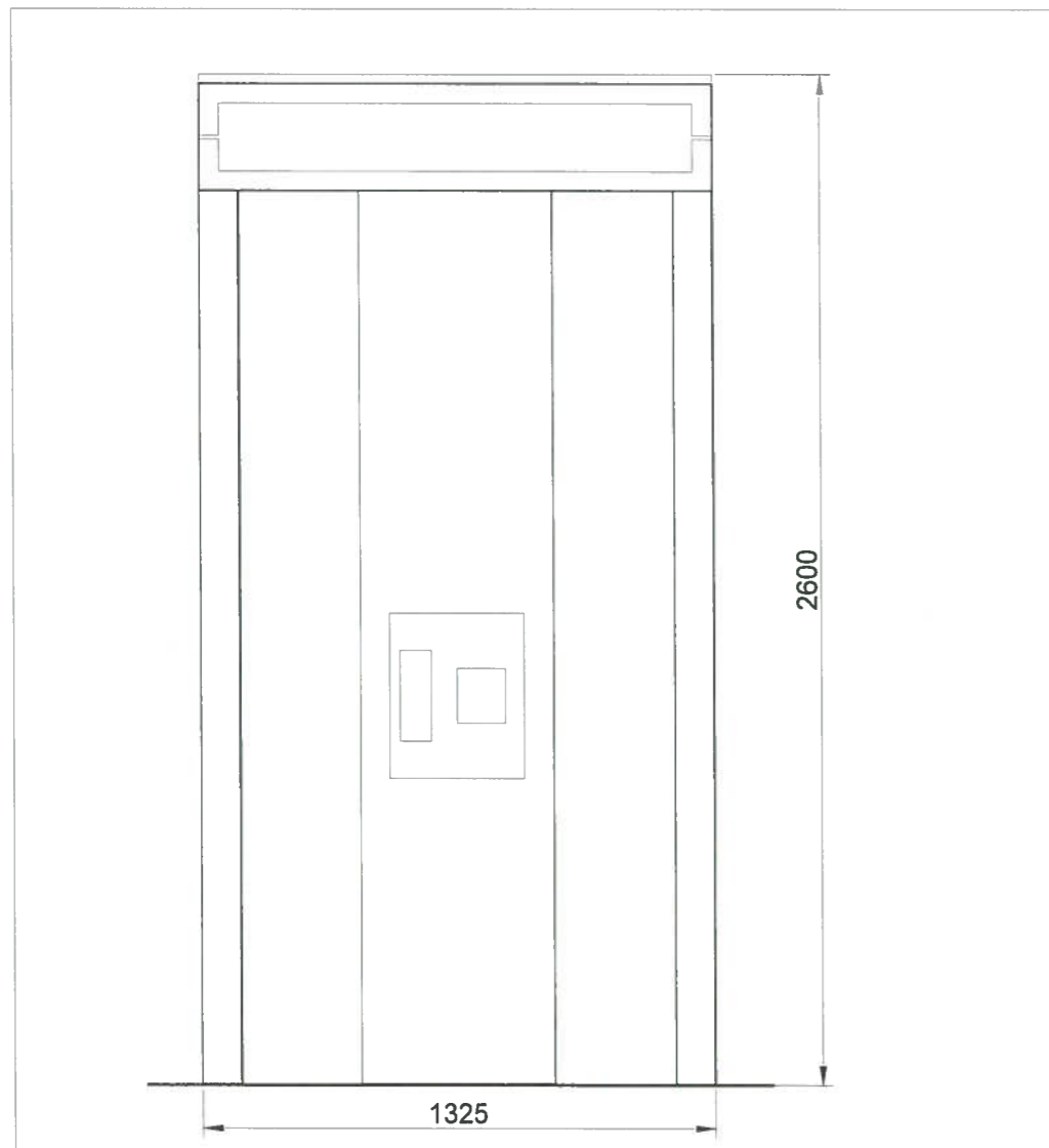
03 Front Elevation
