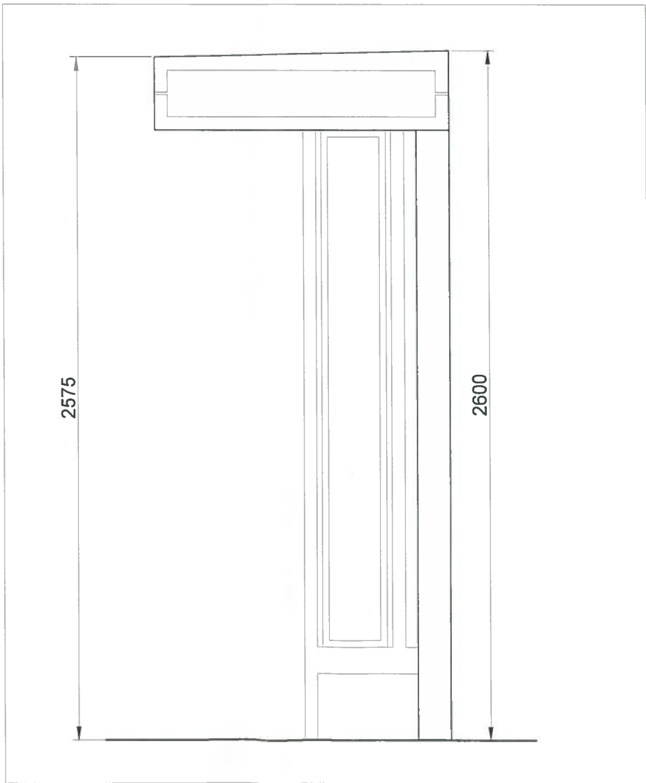
04 Side Elevation
