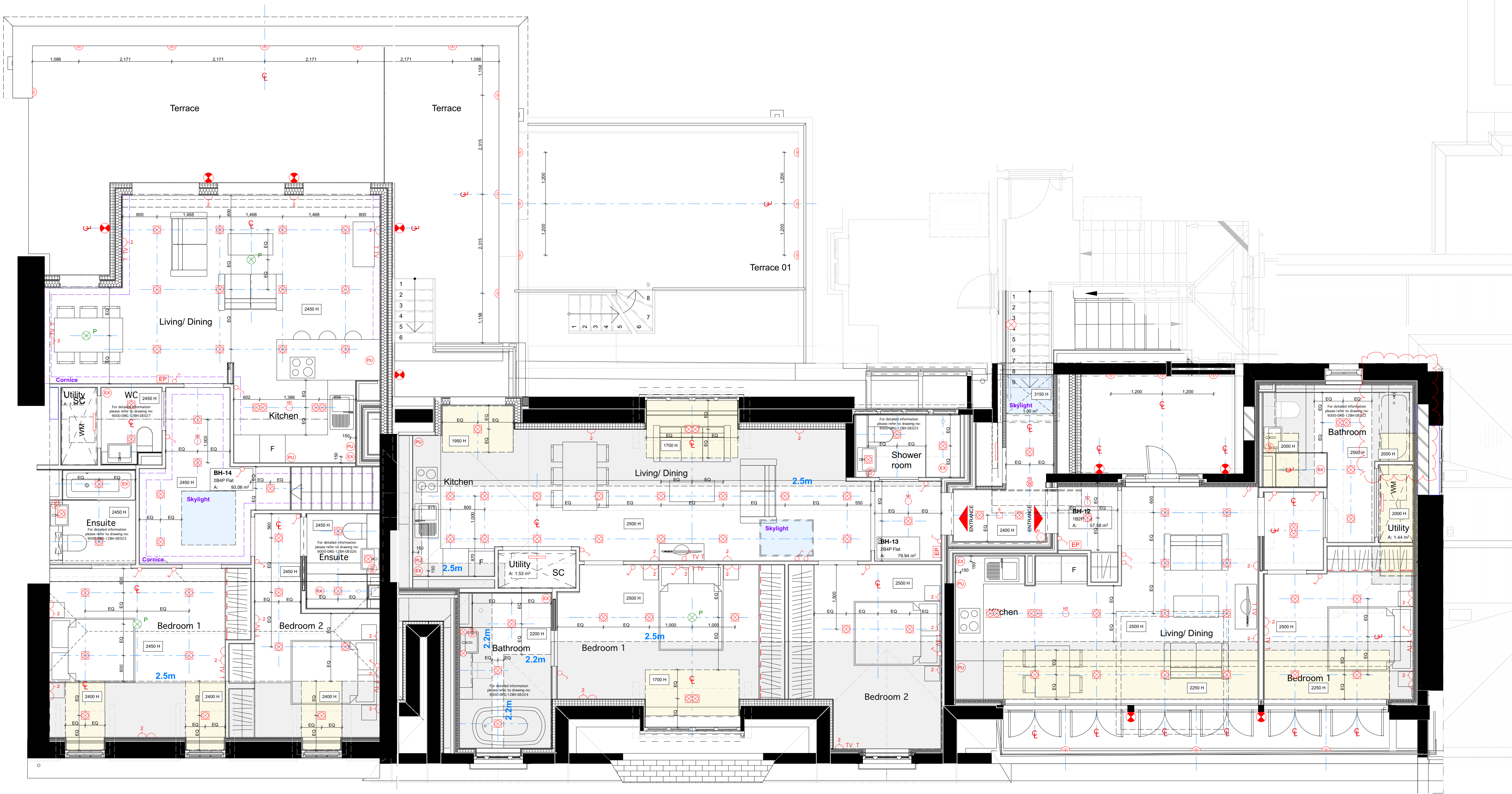
Floor plan cut plane @ 1.5m from FFL
