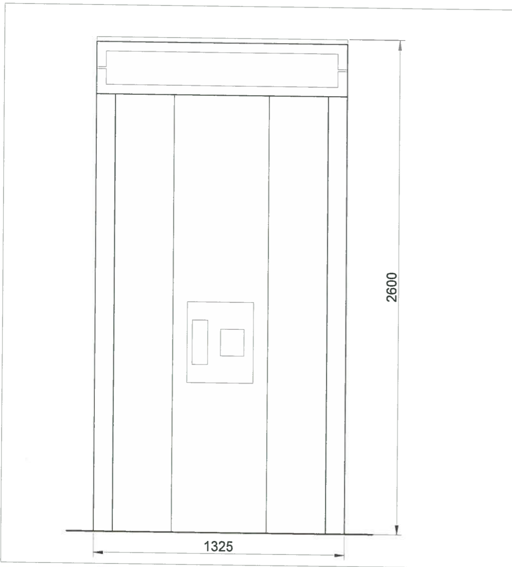
03 Front Elevation
