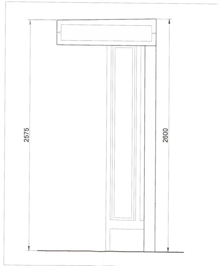
04 Side Elevation
