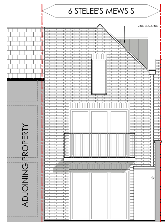
6 COURTYARD GARDEN ELEVATION PROPOSED 1:100
